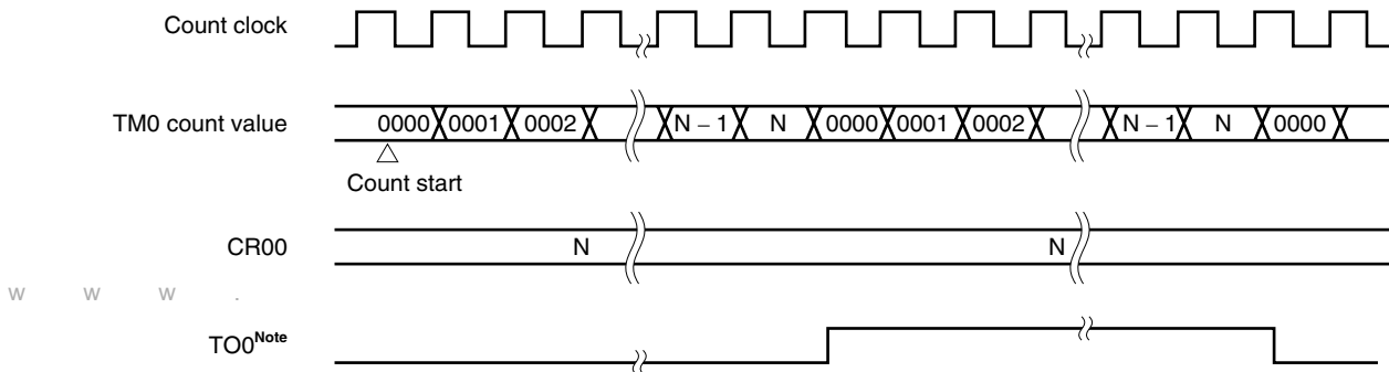
Figure 6-19. Square-Wave Output Operation Timing
