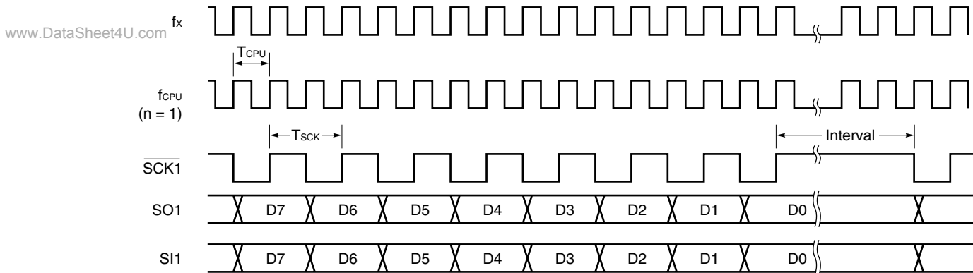
Figure 14-24. Operation Timing When Automatic Transmit/Receive Function Is Operating with Internal Clock
