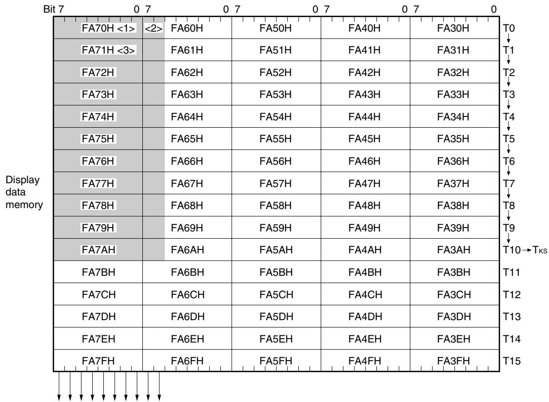
Figure 15-14. Display Data Memory Configuration and Segment Data Reading Order (Segment Type)
