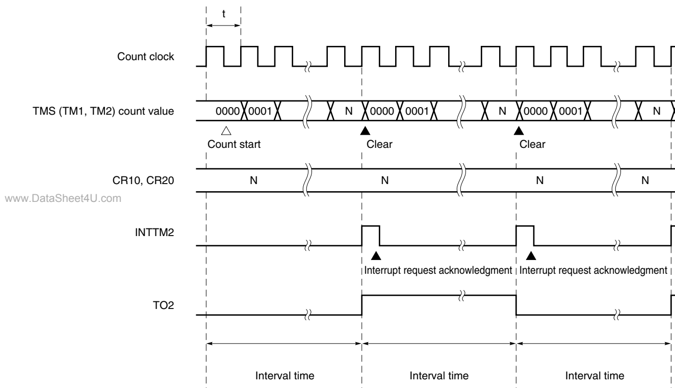
Figure 7-11. Interval Timer Operation Timing
