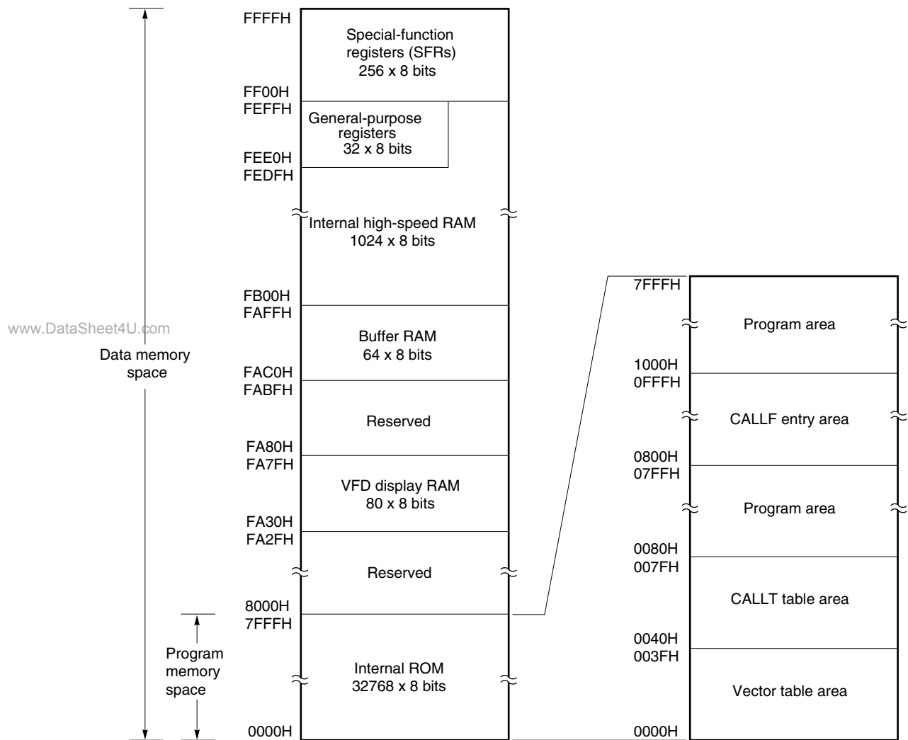
Figure 3-1. Memory Map ( \mu PD780204 and \mu PD780204A)
