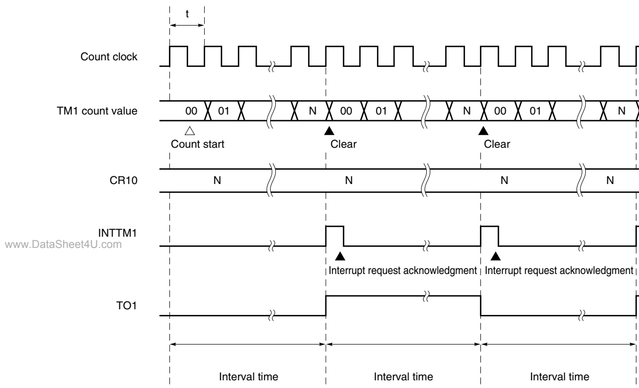
Figure 7-8. Interval Timer Operation Timing
