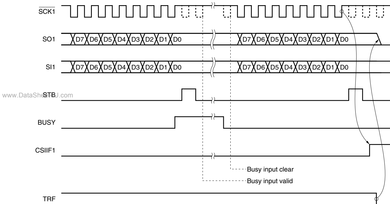
Figure 14-21. Operation Timing When Using Busy & Strobe Control Option (BUSY0 = 0)
