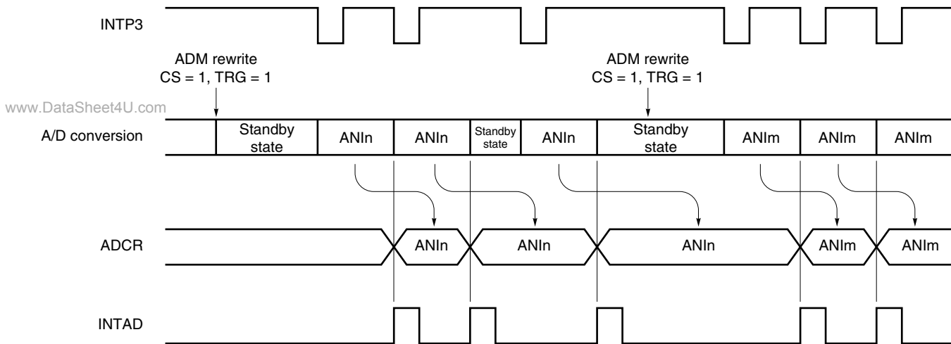
Figure 12-6. A/D Conversion by Hardware Start
