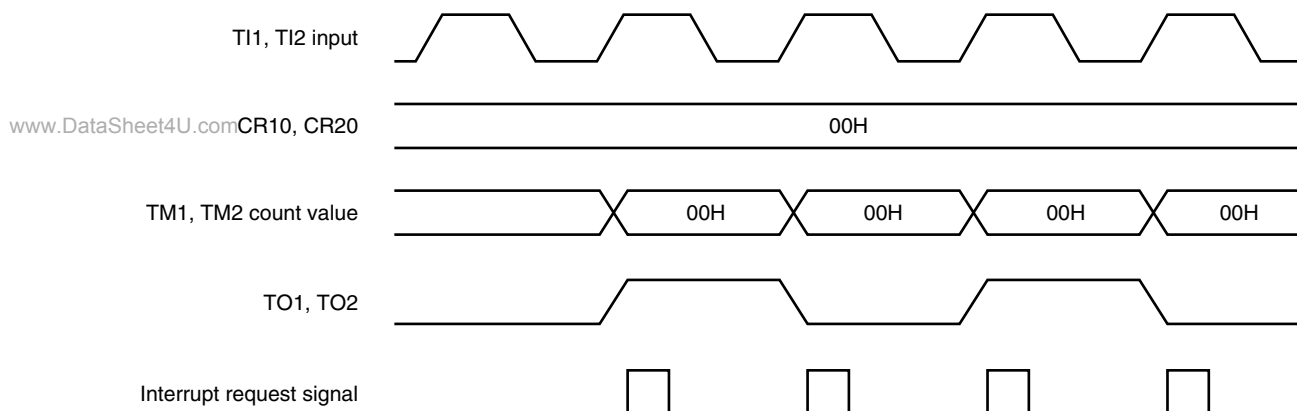
Figure 7-15. External Event Counter Operation Timing
