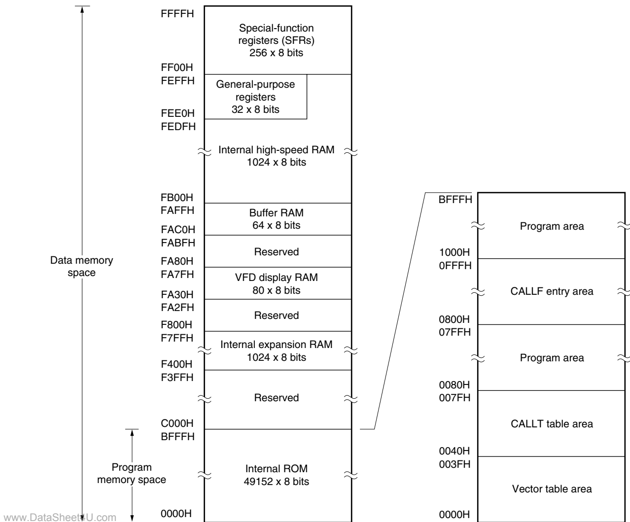
Figure 3-3. Memory Map ( \mu PD780206)
