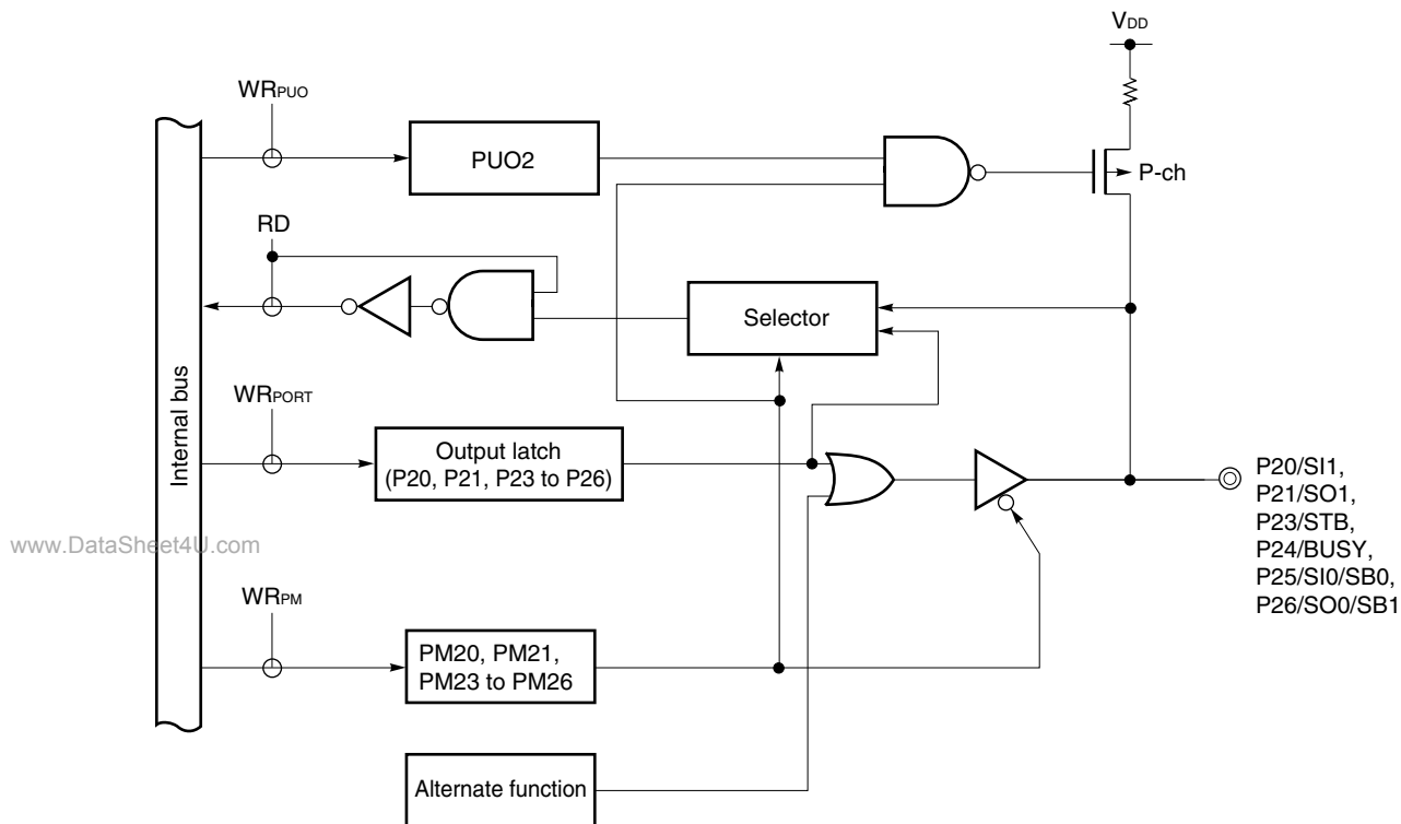
Figure 4-5. Block Diagram of P20, P21, P23 to P26
