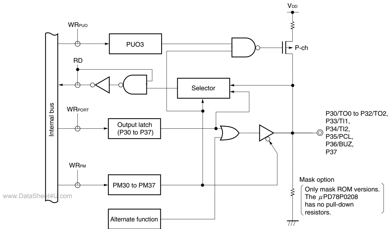
Figure 4-7. Block Diagram of P30 to P37
