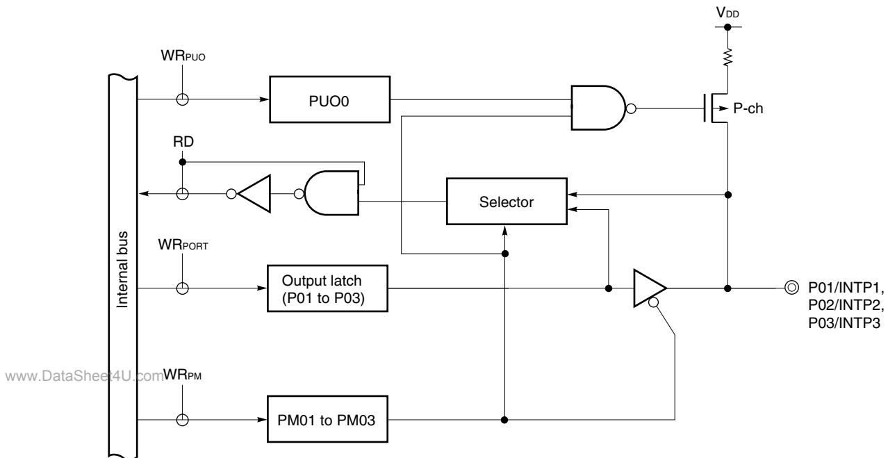
Figure 4-3. Block Diagram of P01 to P03
