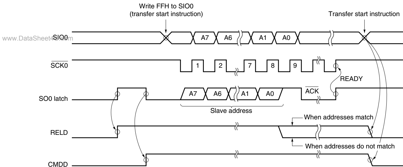
Figure 13-20. RELD and CMDD Operations (Slave)
