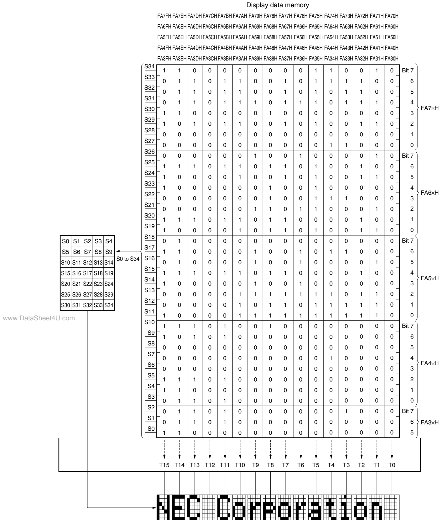
Figure 15-24. Relationship Between Display Data Memory Contents and Segment Outputs in 35-Segment x 16-Digit Display Mode
