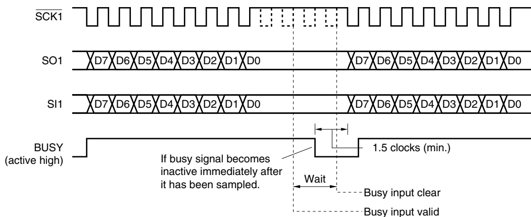
Figure 14-20. Busy Signal and Clearing Wait (BUSY0 = 0)
