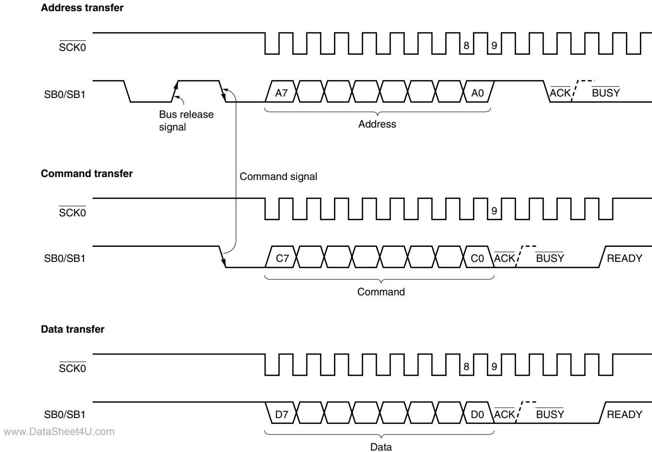
Figure 13-10. SBI Transfer Timing
