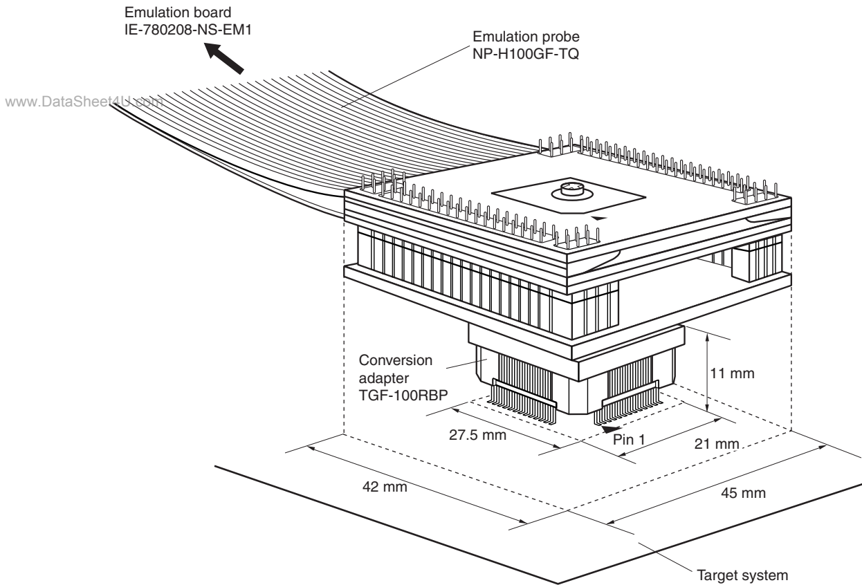
Figure B-6. Connection Conditions of Target System (When NP-H100GF-TQ Is Used)
