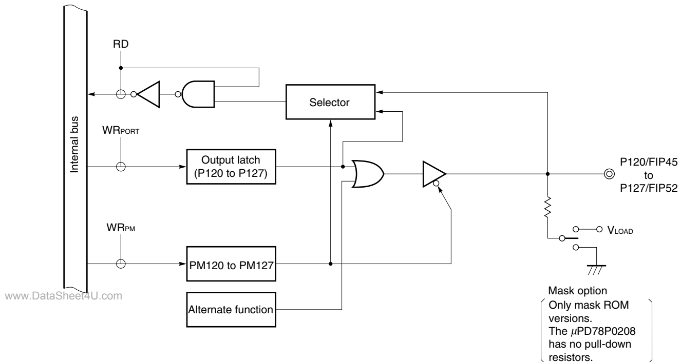
Figure 4-13. Block Diagram of P120 to P127
