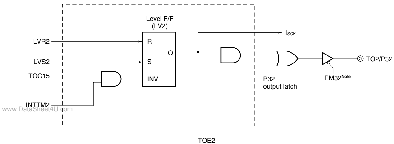
Figure 7-3. Block Diagram of 8-Bit Timer/Event Counter Output Controller 2
