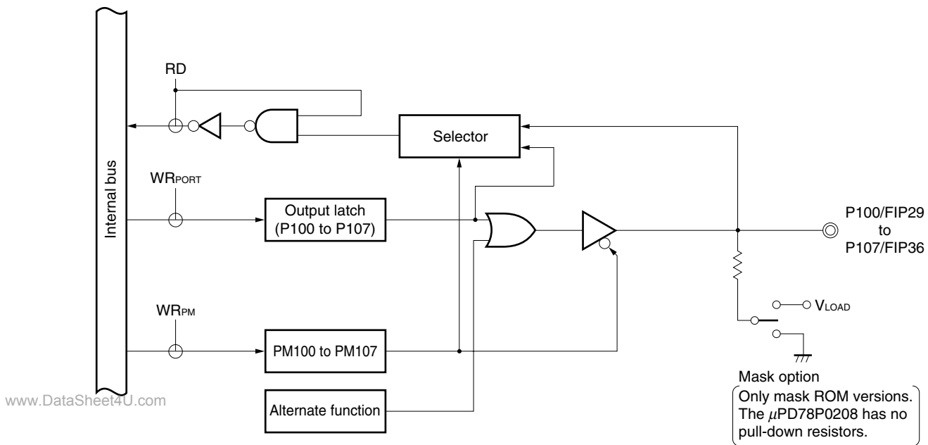
Figure 4-11. Block Diagram of P100 to P107
