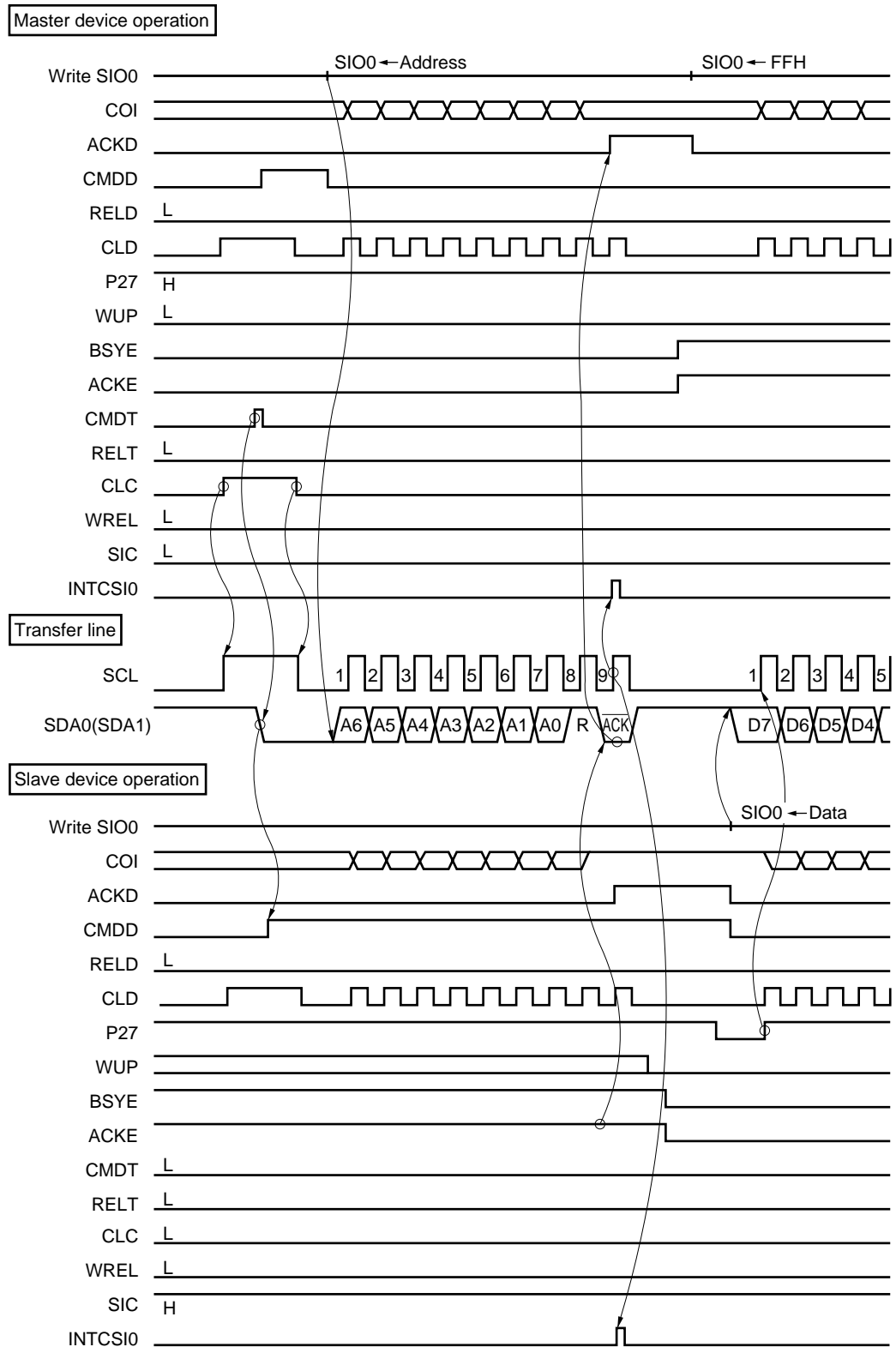
Figure 16-23. Data Transmission from Slave to Master (Both Master and Slave Selected 9-Clock Wait) (1 of 3) (a) Start Condition to Address
