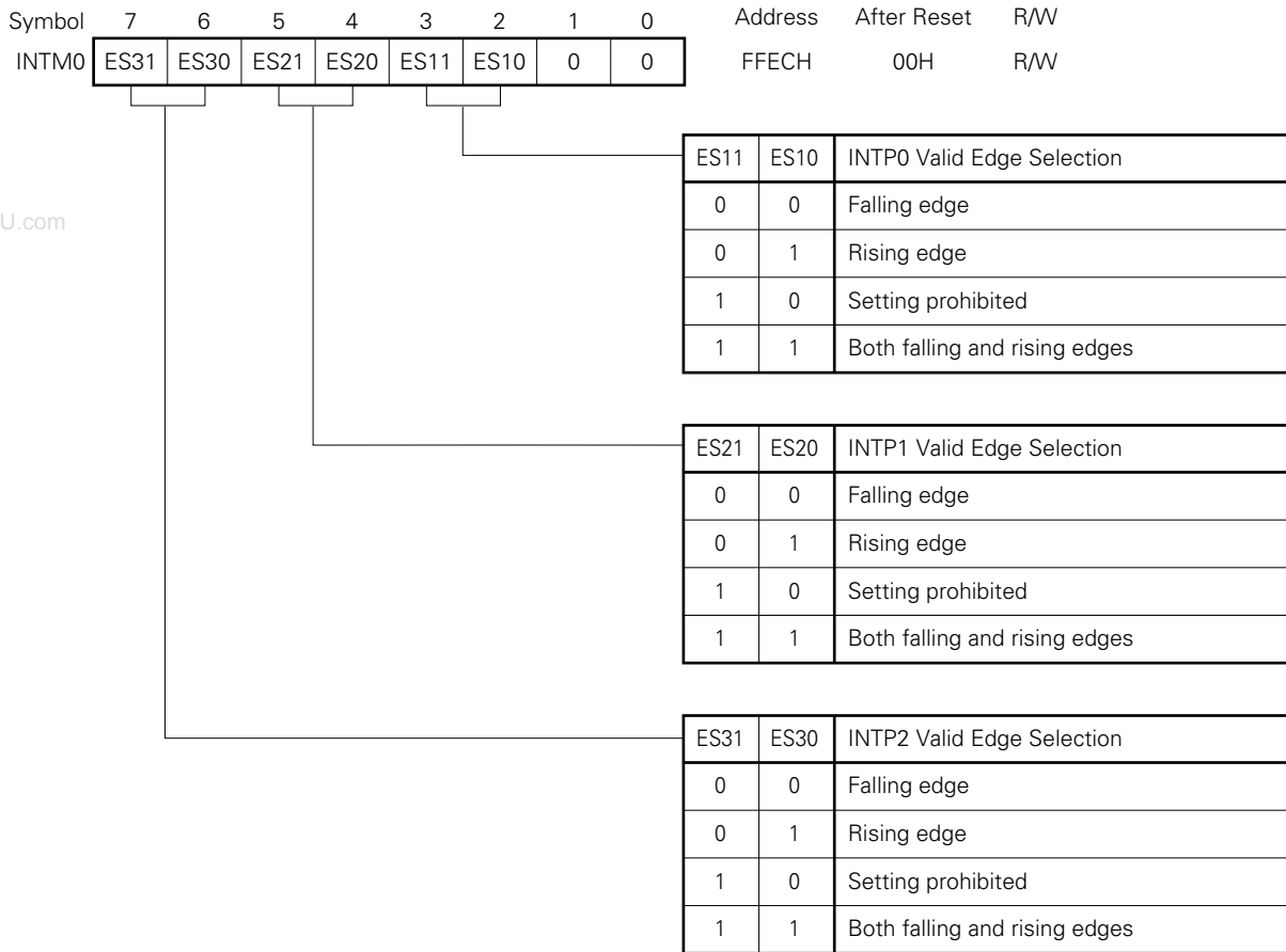
Figure 8-8. External Interrupt Mode Register 0 Format
