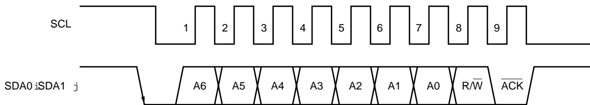
Figure 16-18. Acknowledge Signal
