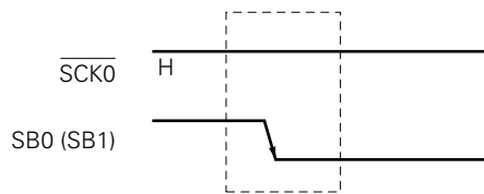
Figure 15-13. Command Signal
