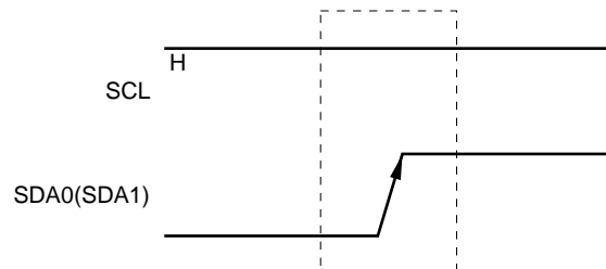
Figure 16-19. Stop Condition
