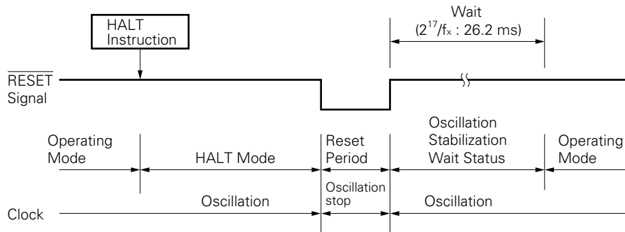
Figure 20-3. HALT Mode Release by \overline{\text{RESET}} Input
