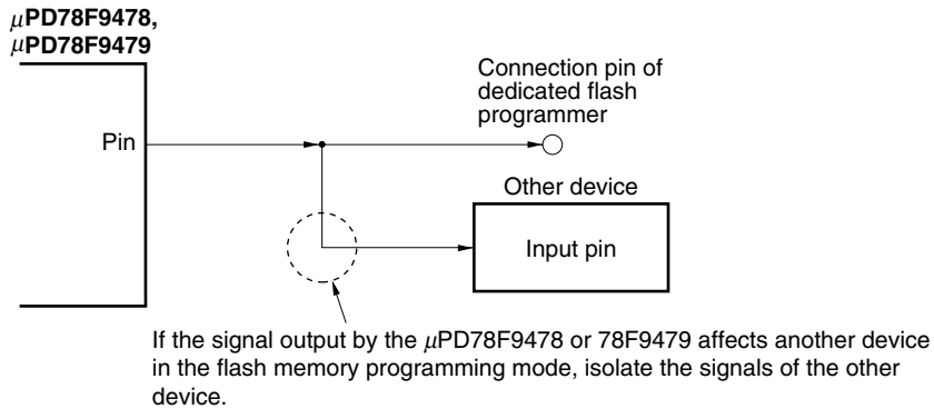
Figure 19-6. Abnormal Operation of Other Device
