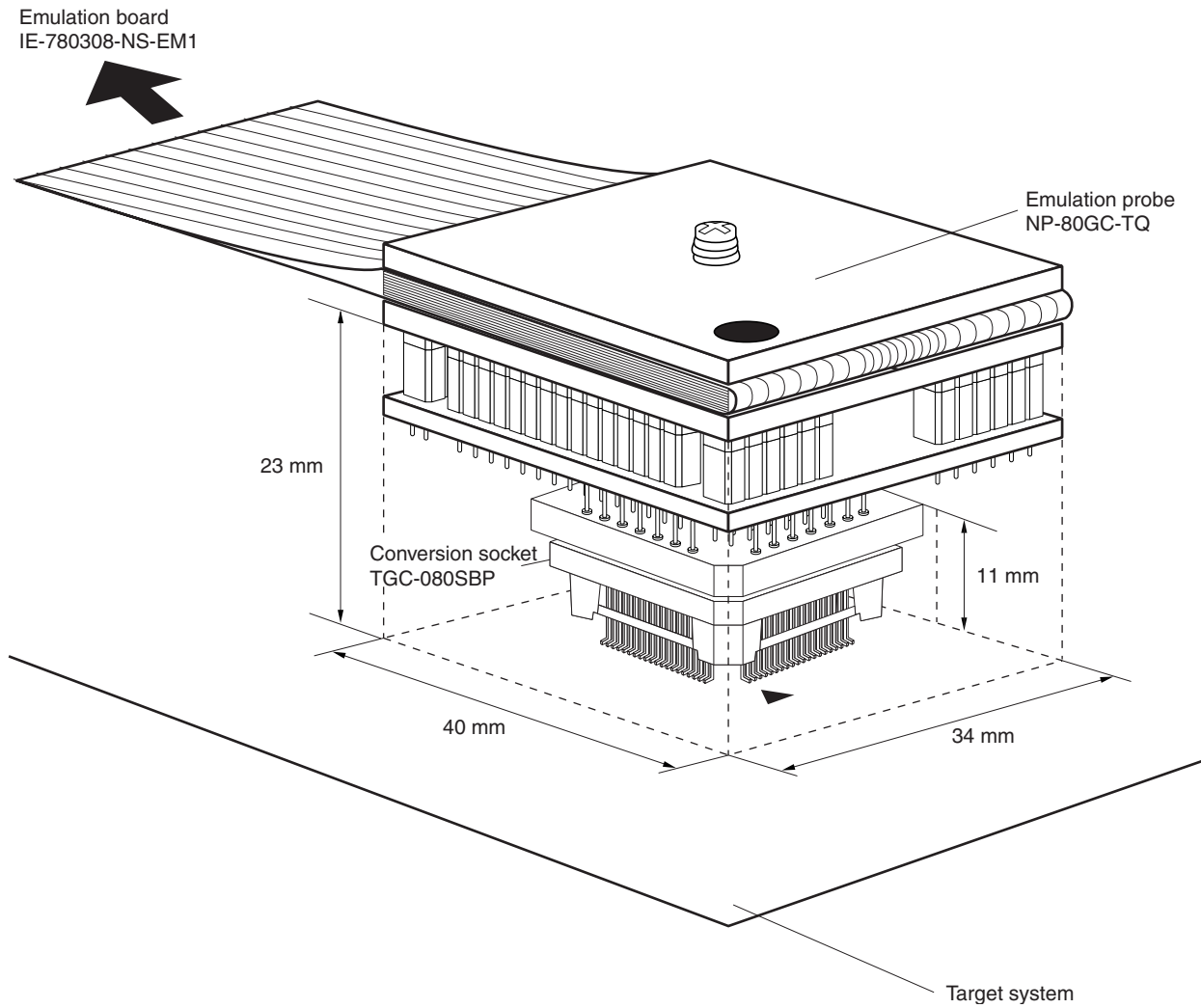
Figure B-7. Connection Condition of Target System (NP-80GC-TQ)
