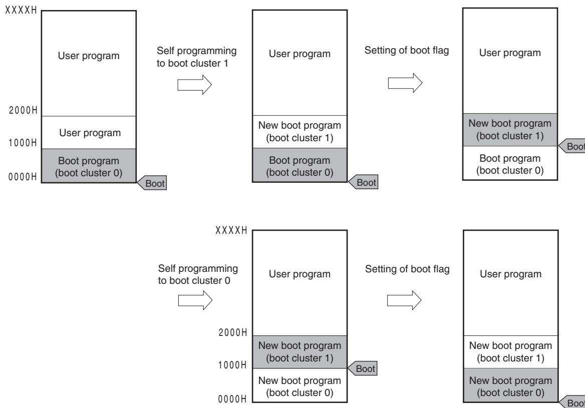
<R> Figure 25-21. Boot Swap Function
