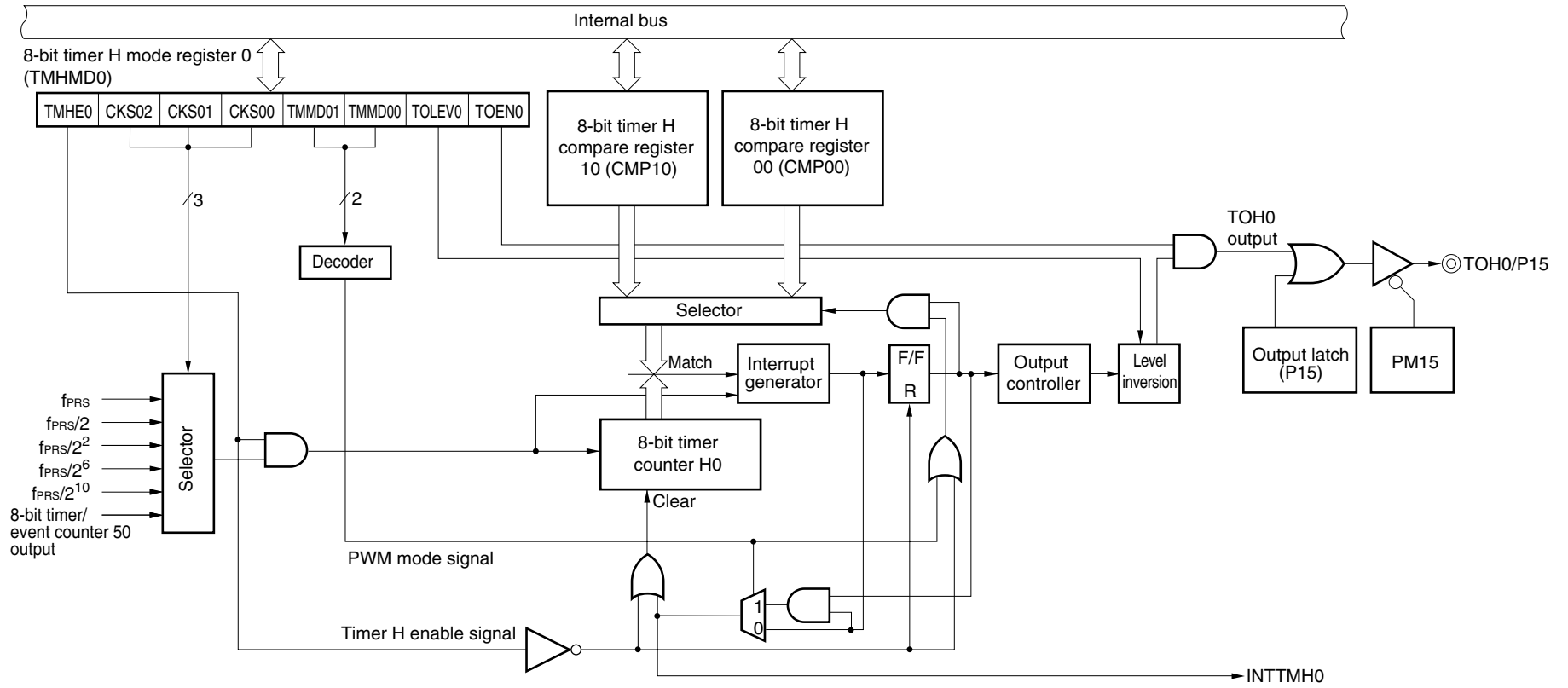
<R> Figure 8-1. Block Diagram of 8-bit Timer H0
