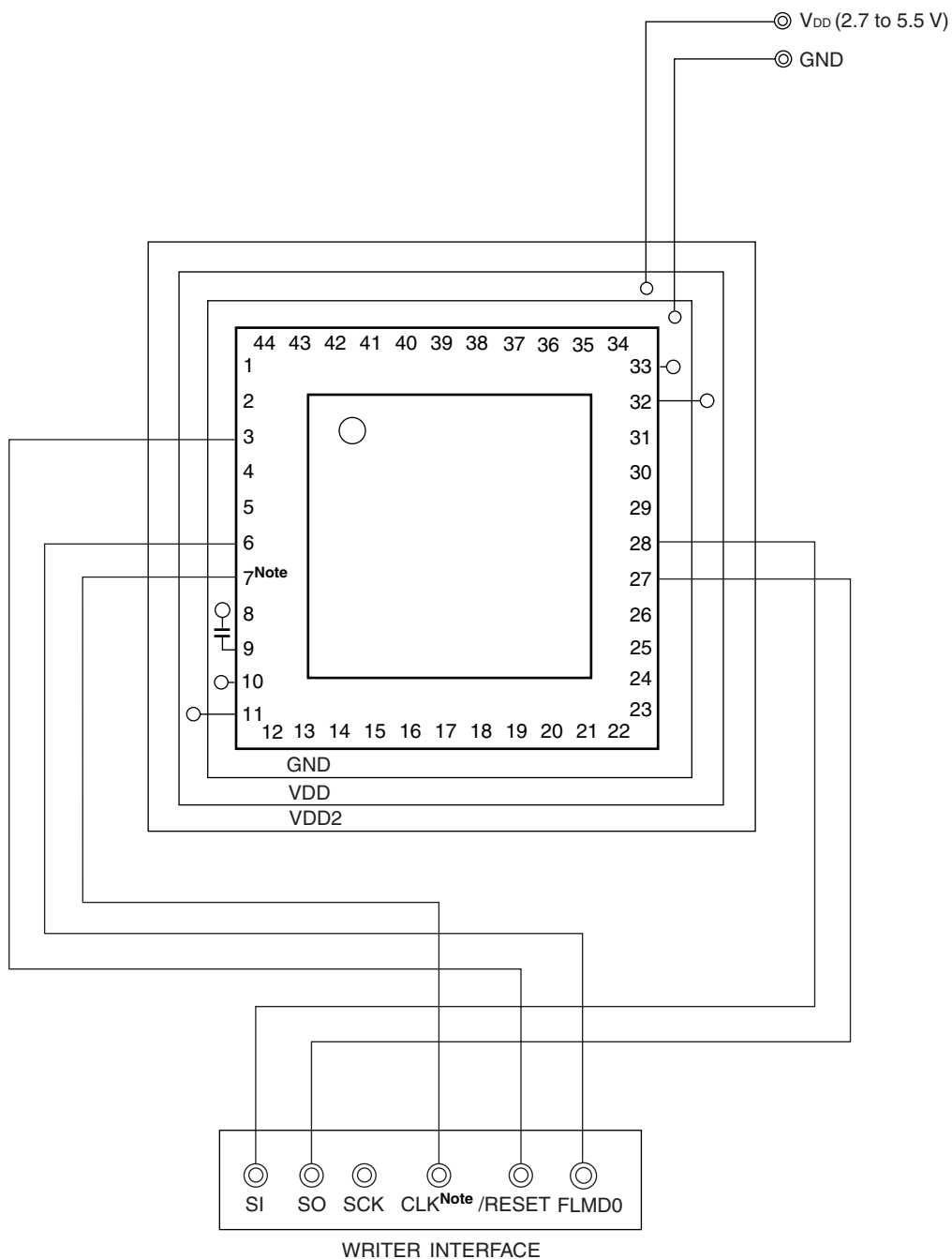
Figure 25-6. Example of Wiring Adapter for Flash Memory Writing in UART (UART6) Mode (44-Pin Products)
