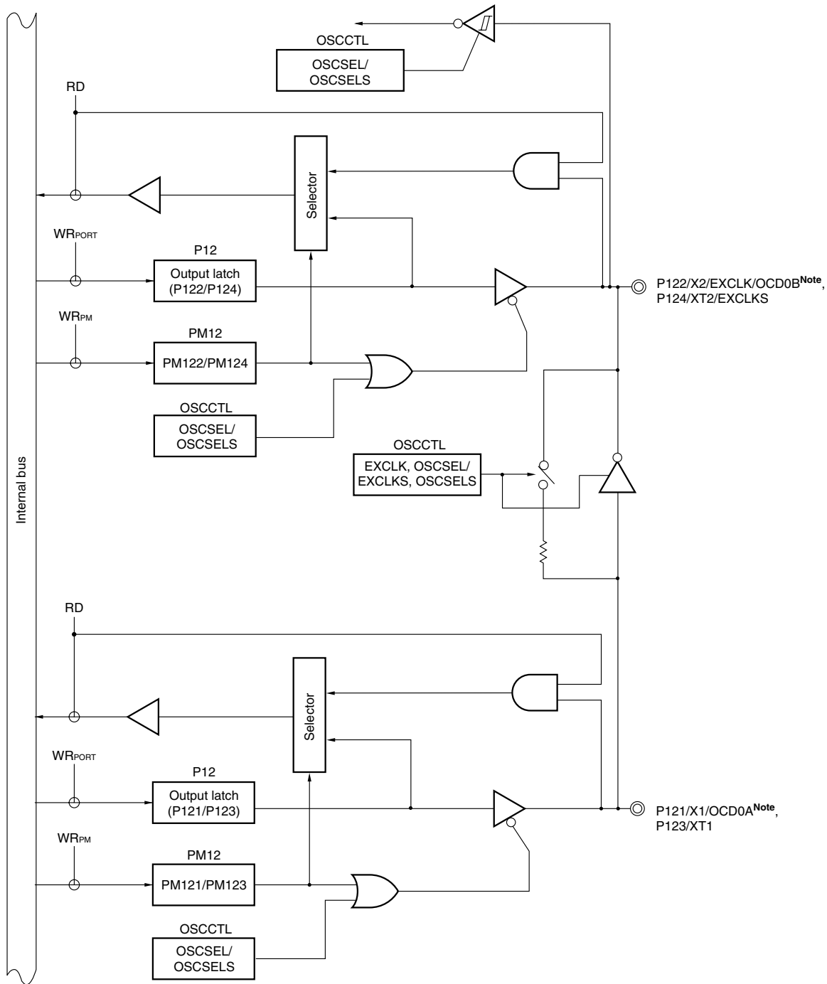
Figure 4-18. Block Diagram of P121 to P124
