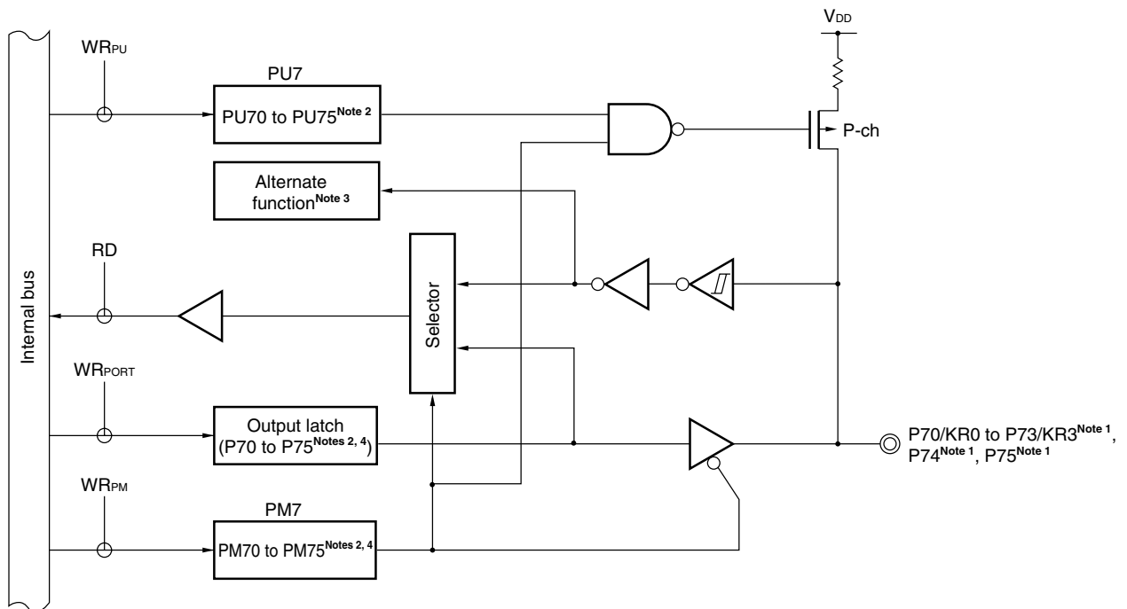
Figure 4-16. Block Diagram of P70 to P75
