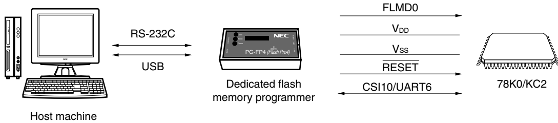
Figure 25-9. Environment for Writing Program to Flash Memory
