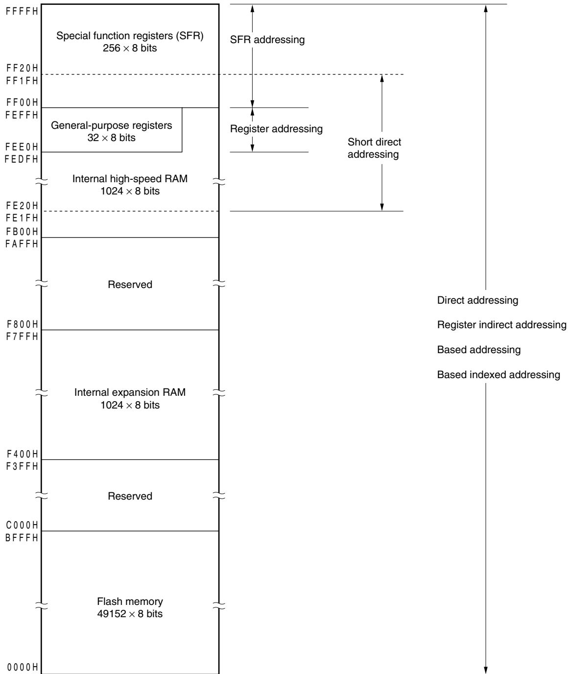
Figure 3-11 . Correspondence Between Data Memory and Addressing ( \mu PD78F0514)
