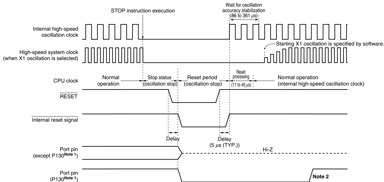
Figure 21-4. Timing of Reset in STOP Mode by RESET Input
