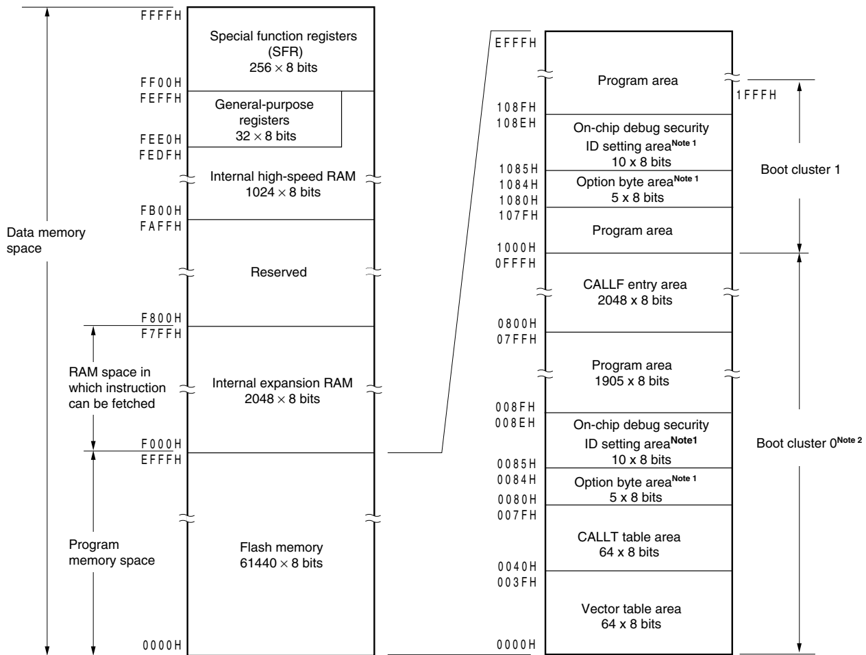
Figure 3-7. Memory Map ( \mu PD78F0515D)
