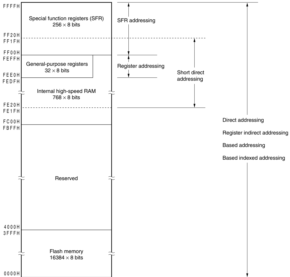
Figure 3-8. Correspondence Between Data Memory and Addressing ( \mu PD78F0511)
