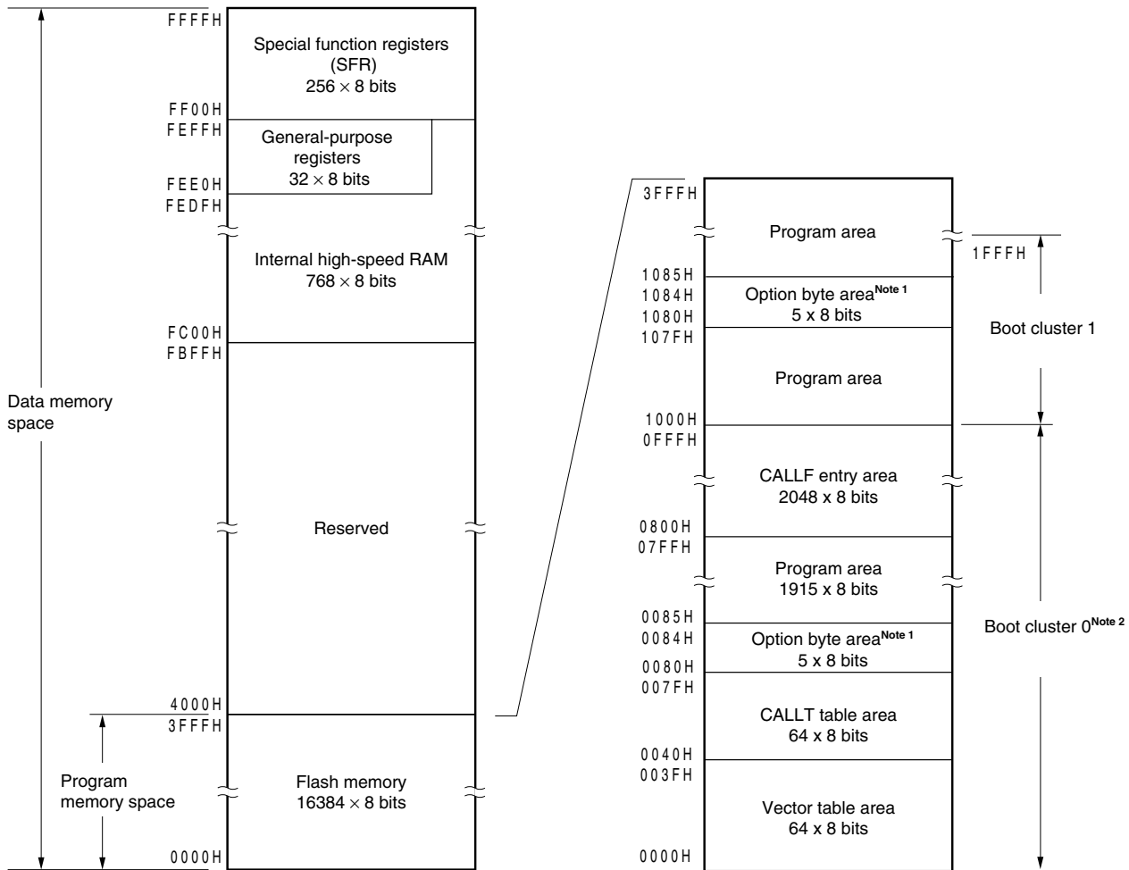
Figure 3-1. Memory Map ( \mu PD78F0511)
