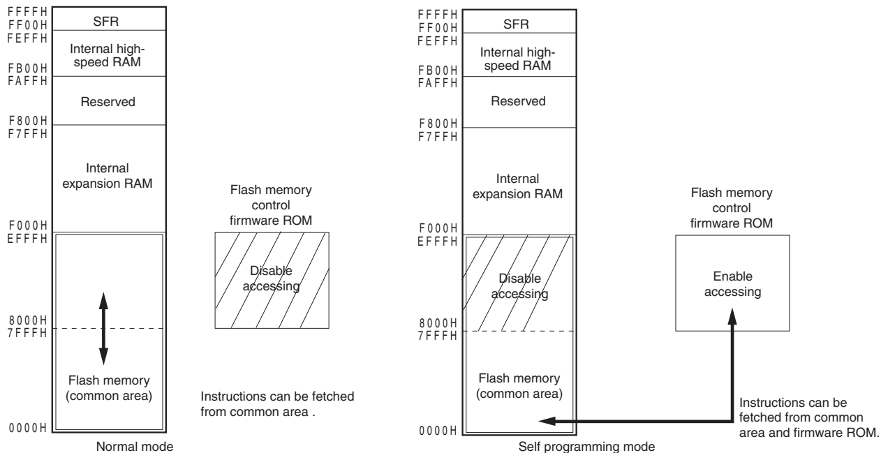
Figure 25-19. Operation Mode and Memory Map for Self Programming ( \mu PD78F0515)
