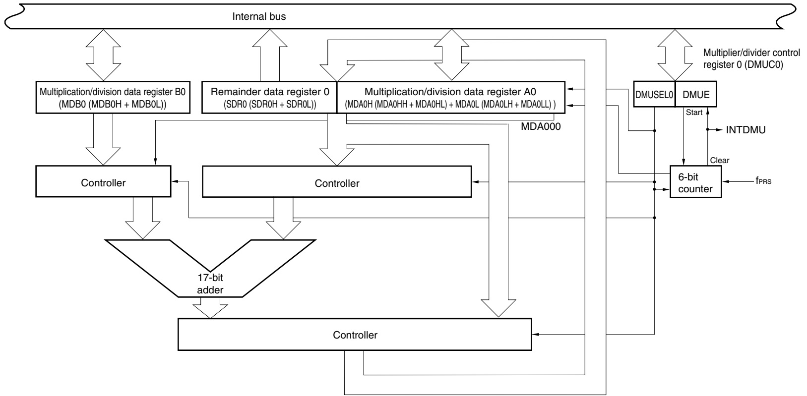
<R> Figure 17-1. Block Diagram of Multiplier/Divider
