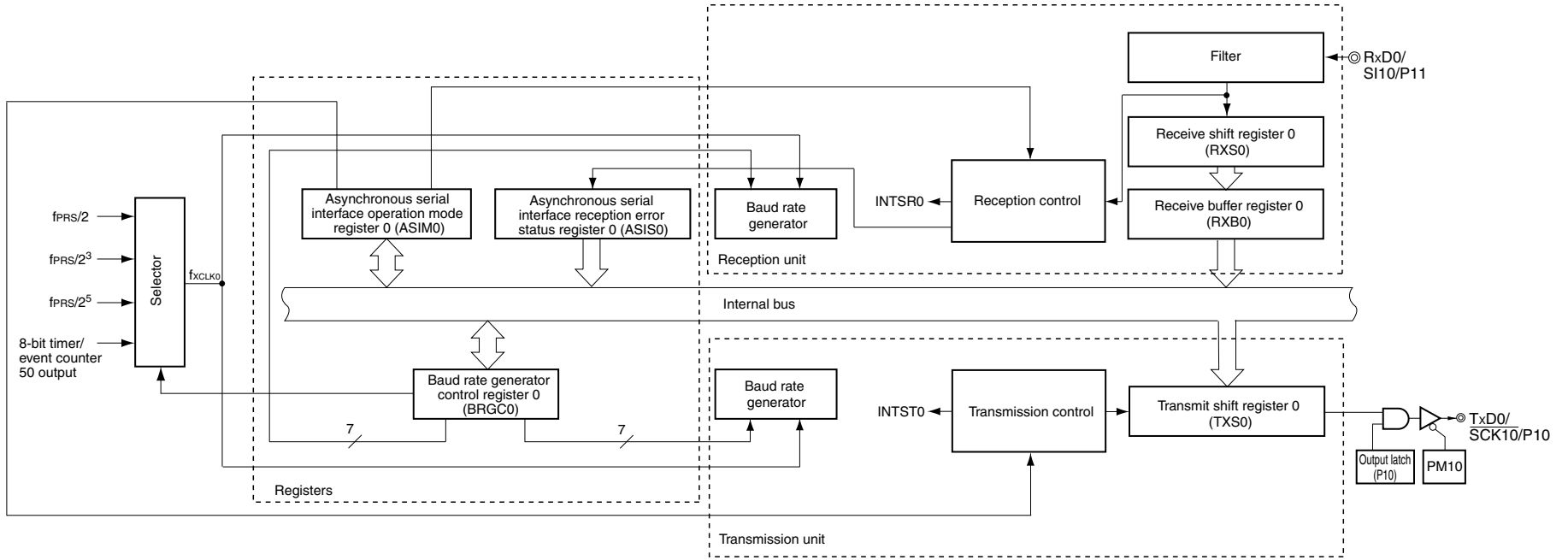
<R> Figure 13-1. Block Diagram of Serial Interface UART0
