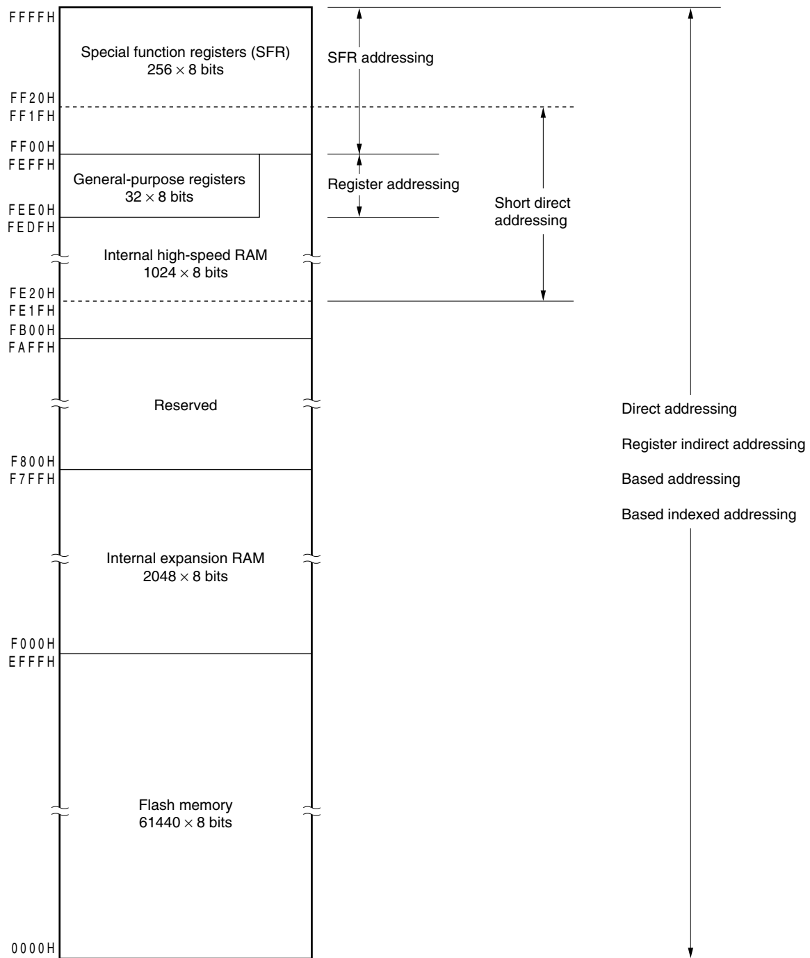
Figure 3-12. Correspondence Between Data Memory and Addressing ( \mu PD78F0515 and 78F0515D)
