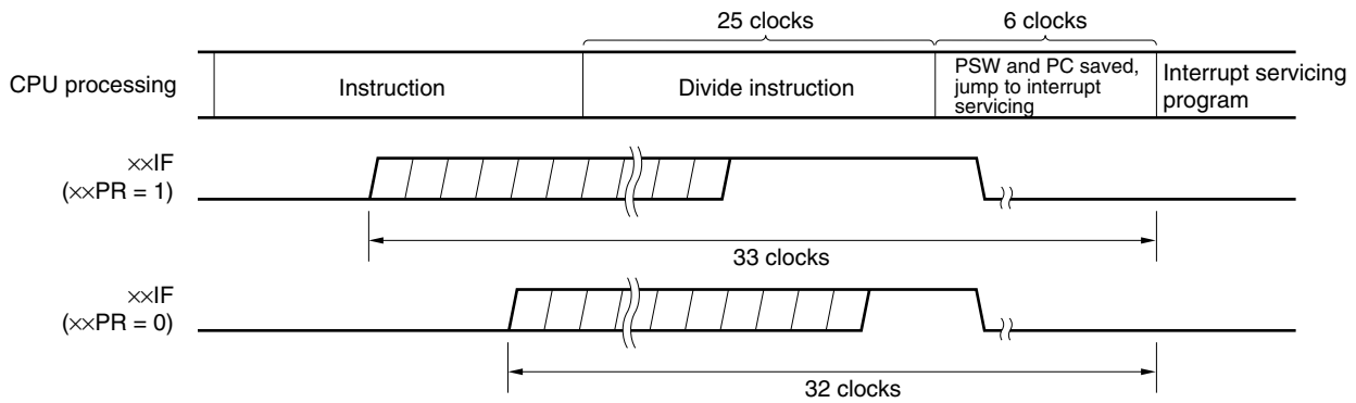
Figure 18-9. Interrupt Request Acknowledgment Timing (Maximum Time)
