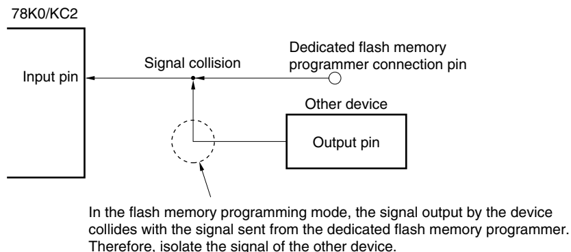
Figure 25-13. Signal Collision (Input Pin of Serial Interface)
