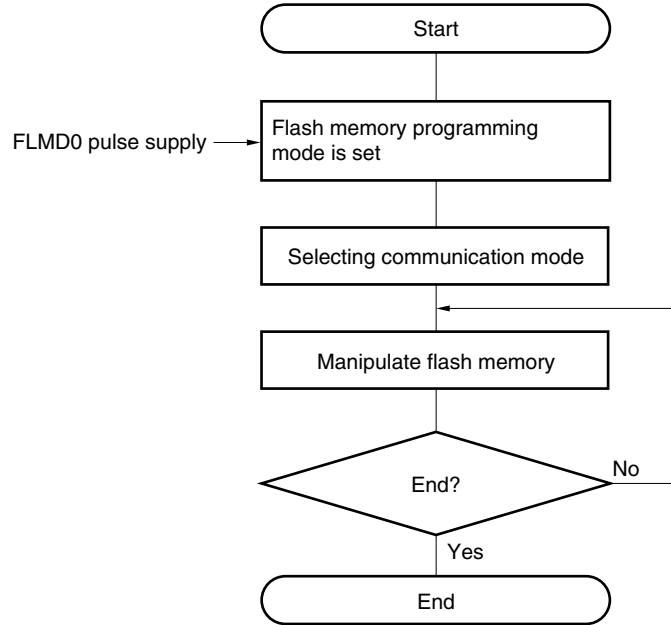
Figure 25-16. Flash Memory Manipulation Procedure
