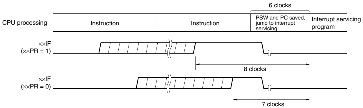
Figure 18-8. Interrupt Request Acknowledgment Timing (Minimum Time)
