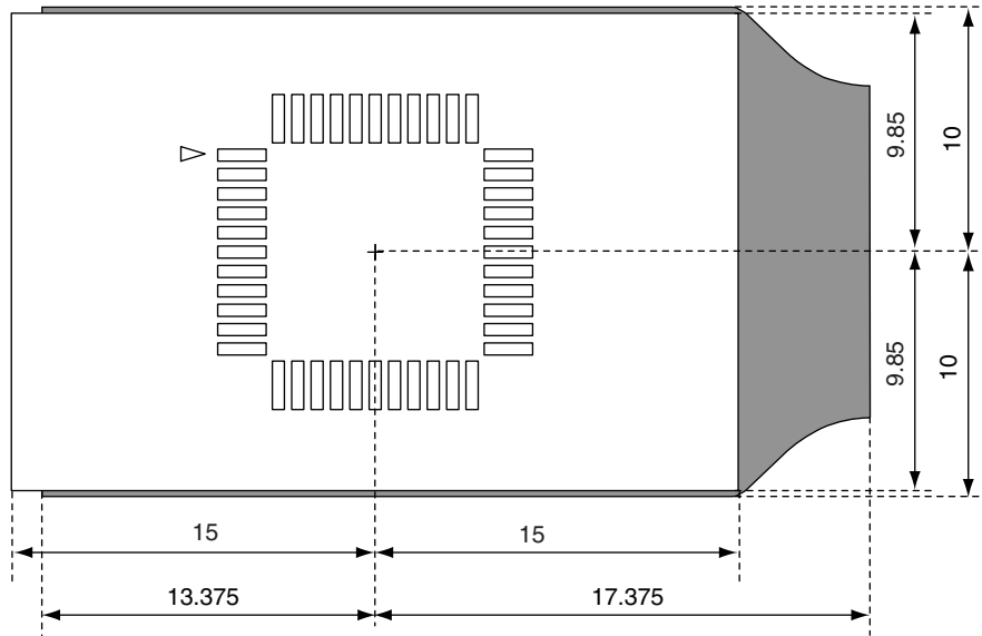
Figure B-1. For 44-Pin GB Package
