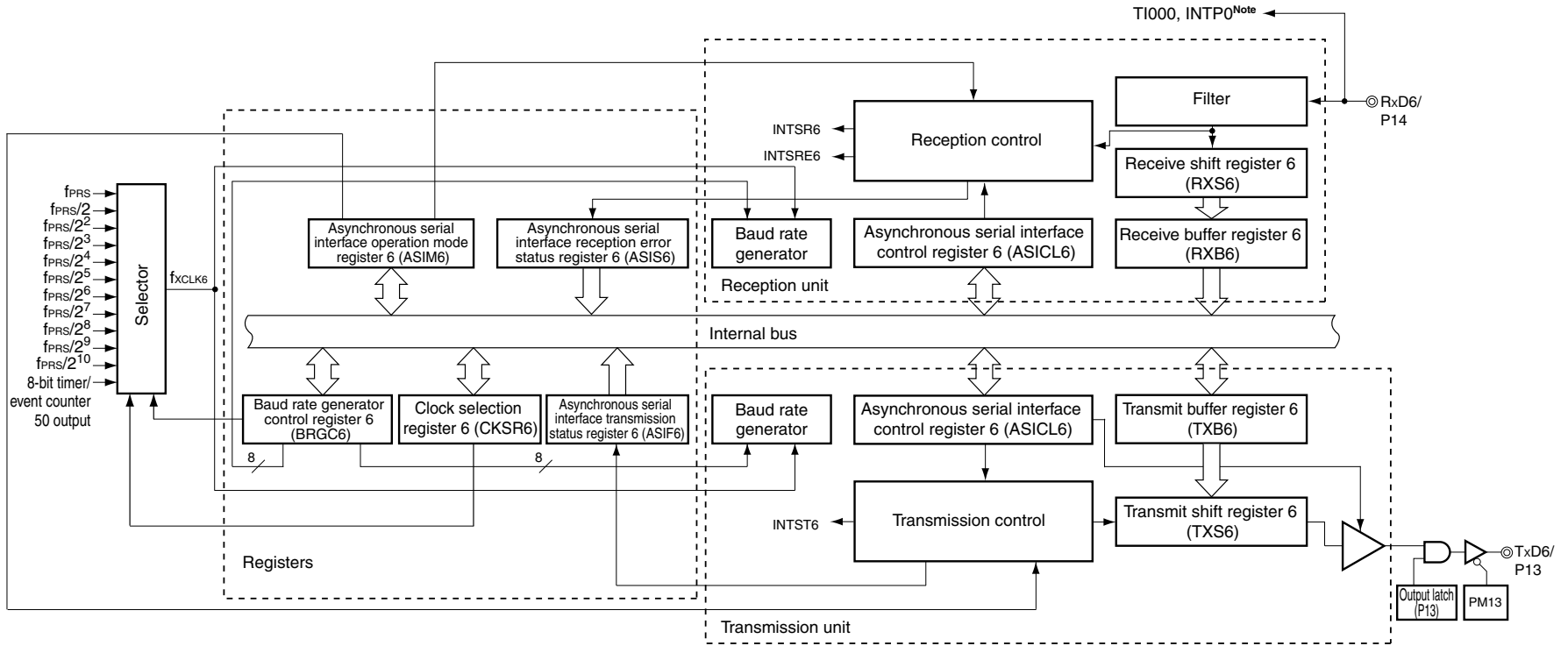
<R>Figure 14-4. Block Diagram of Serial Interface UART6
