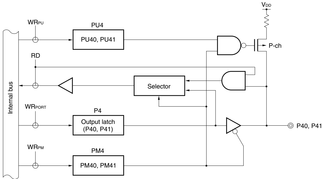
Figure 4-12. Block Diagram of P40, P41 (44-Pin and 48-Pin Products Only)
