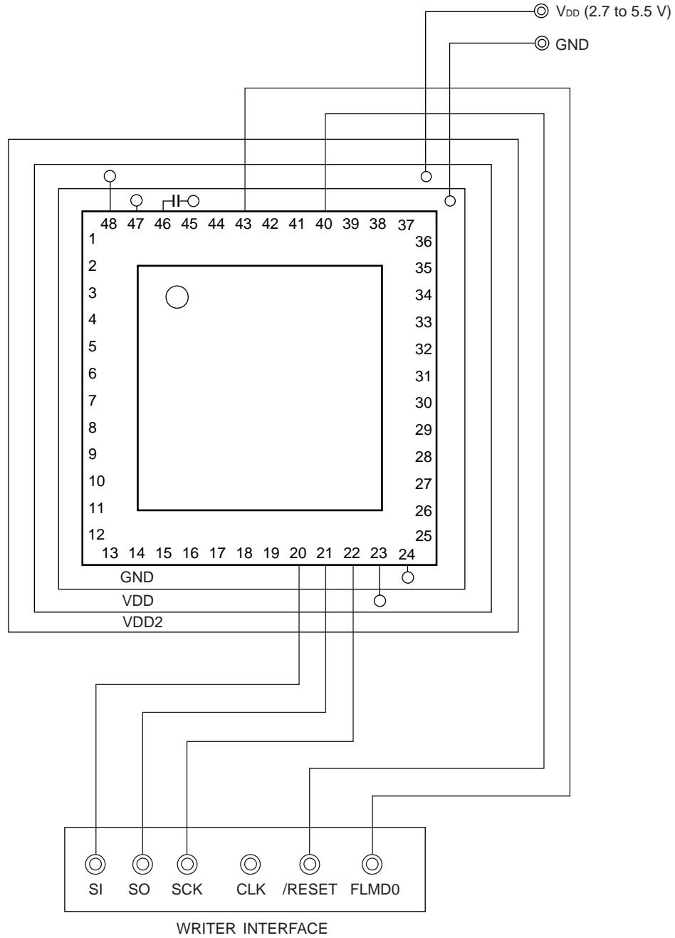
Figure 25-7. Example of Wiring Adapter for Flash Memory Writing in 3-Wire Serial I/O (CSI10) Mode (48-Pin Products)
