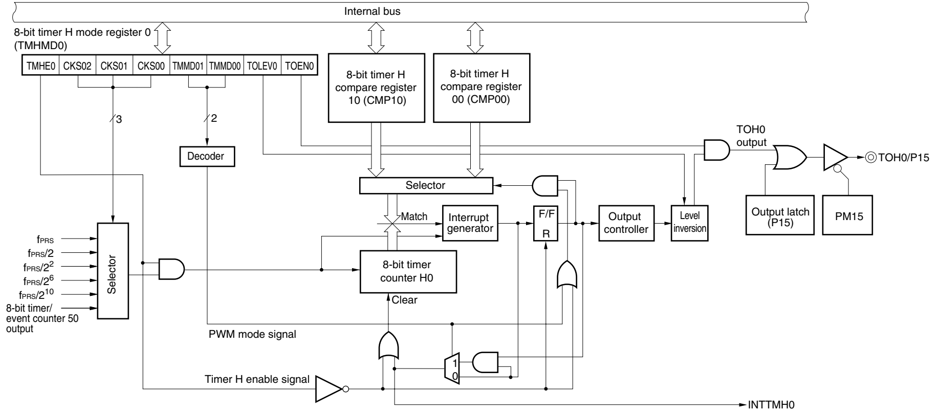
<R> Figure 8-1. Block Diagram of 8-bit Timer H0
