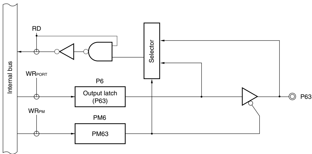
Figure 4-15. Block Diagram of P63
