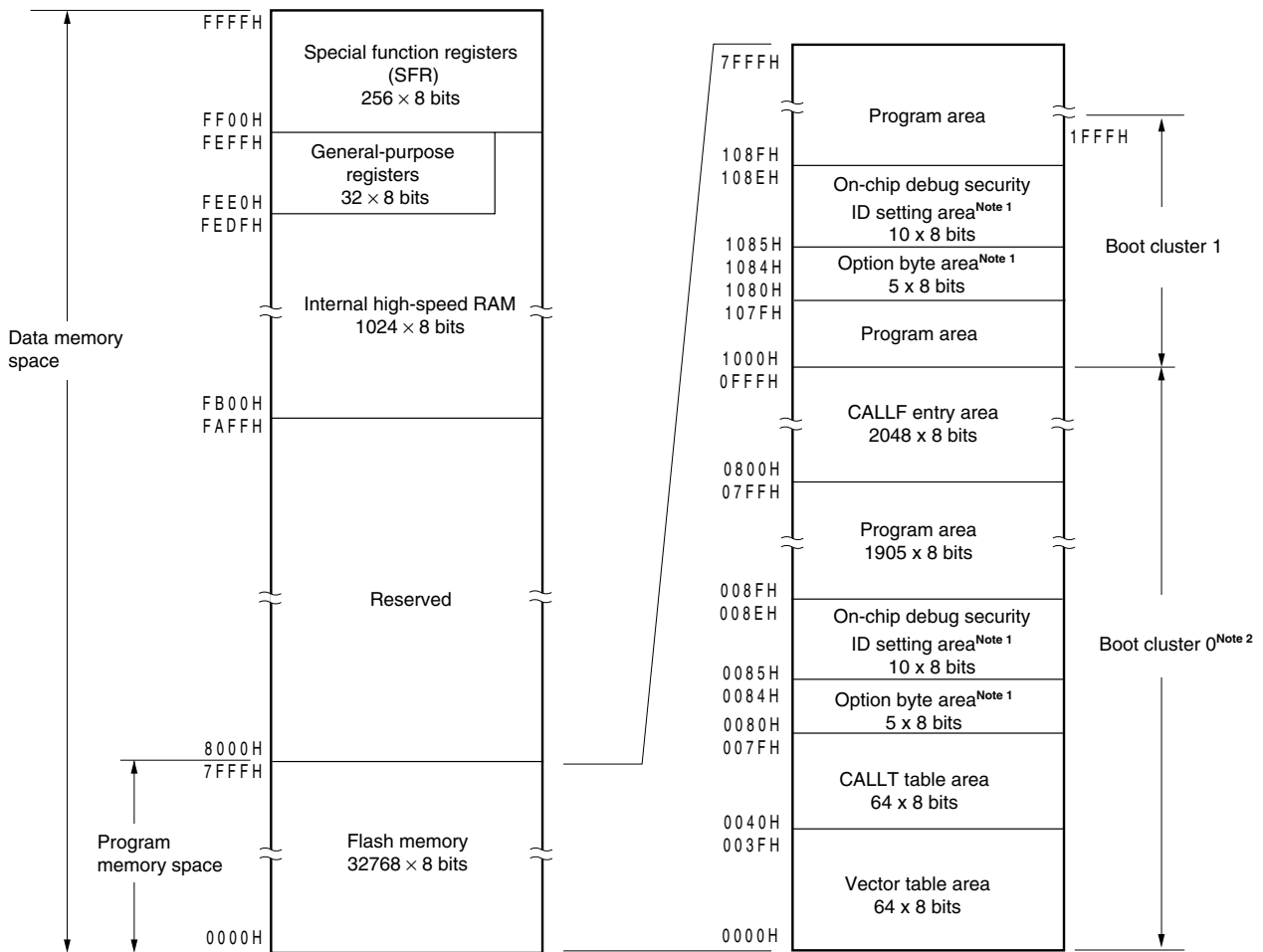
Figure 3-4. Memory Map ( \mu PD78F0513D)
