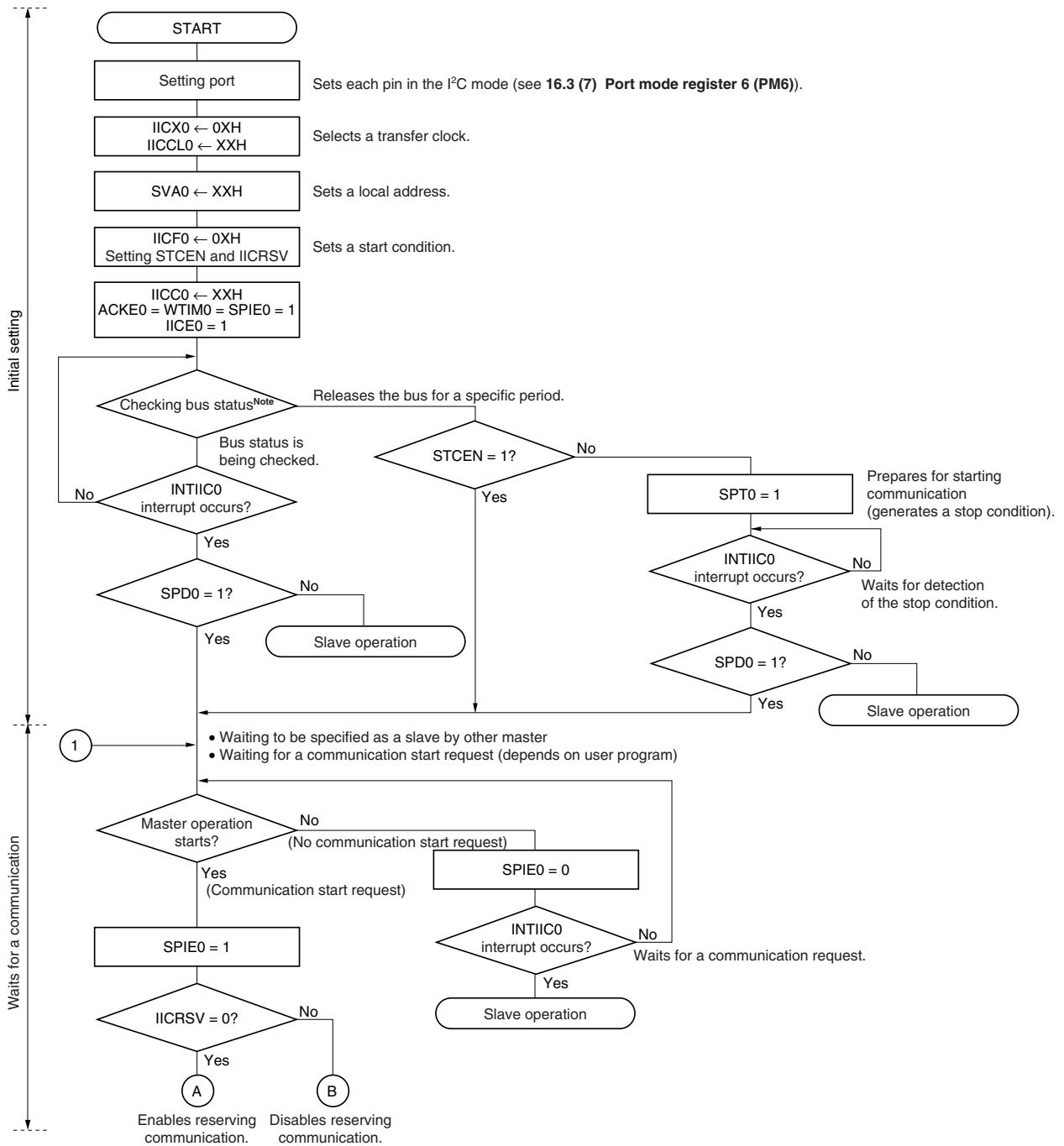
Figure 16-24. Master Operation in Multi-Master System (1/3)
