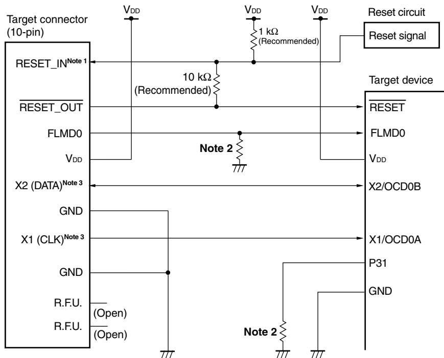
Figure 26-1. Connection Example of QB-78K0MINI or QB-MINI2 and \mu PD78F0513D, 78F0515D (When OCD0A/X1 and OCD0B/X2 Are Used)
