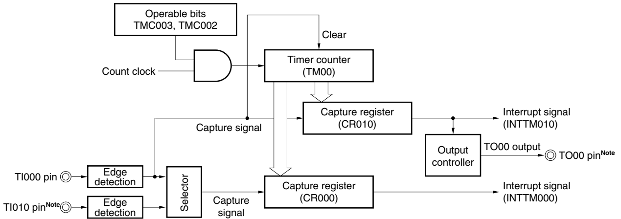
<R> Figure 6-28. Block Diagram of Clear & Start Mode Entered by TI000 Pin Valid Edge Input (CR000: Capture Register, CR010: Capture Register)
