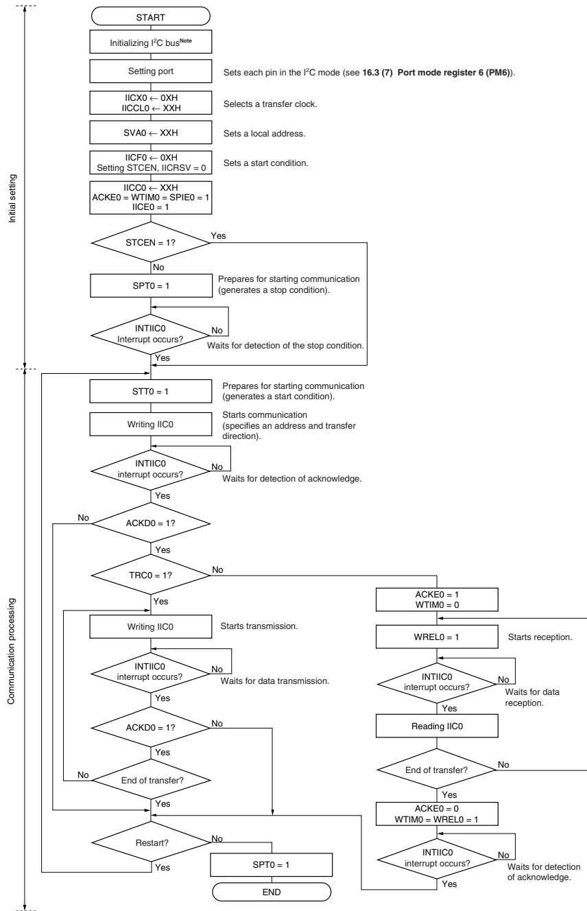
Figure 16-23. Master Operation in Single-Master System
