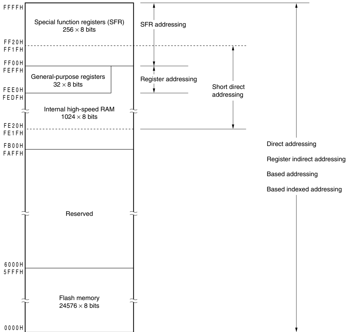
Figure 3-9. Correspondence Between Data Memory and Addressing ( \mu PD78F0512)
