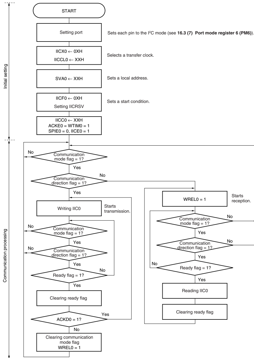
Figure 16-25. Slave Operation Flowchart (1)
