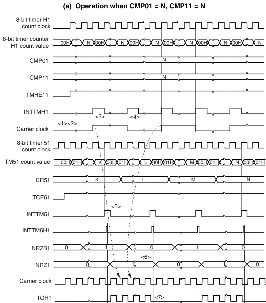
Figure 8-15. Carrier Generator Mode Operation Timing (1/3)
