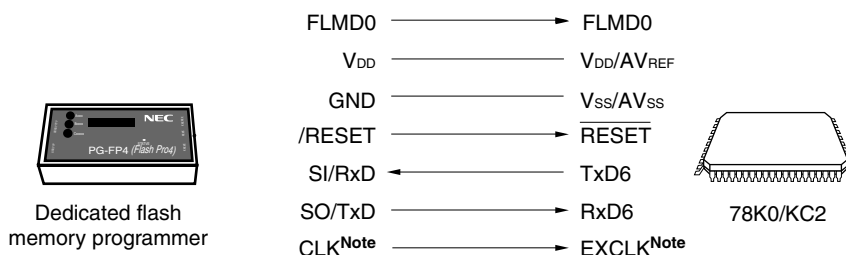
Figure 25-11. Communication with Dedicated Flash Memory Programmer (UART6)
