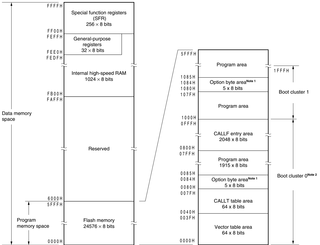
Figure 3-2. Memory Map ( \mu PD78F0512)
