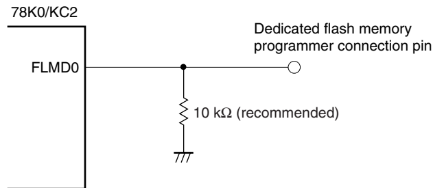
Figure 25-12. FLMD0 Pin Connection Example
