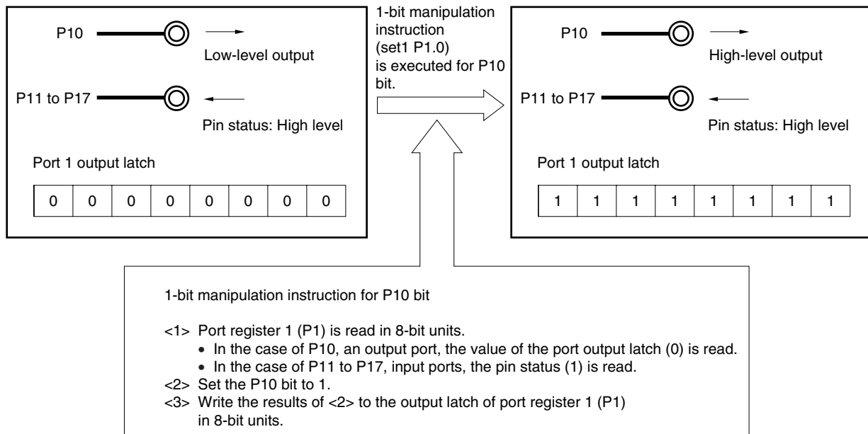
Figure 4-25. Bit Manipulation Instruction (P10)
