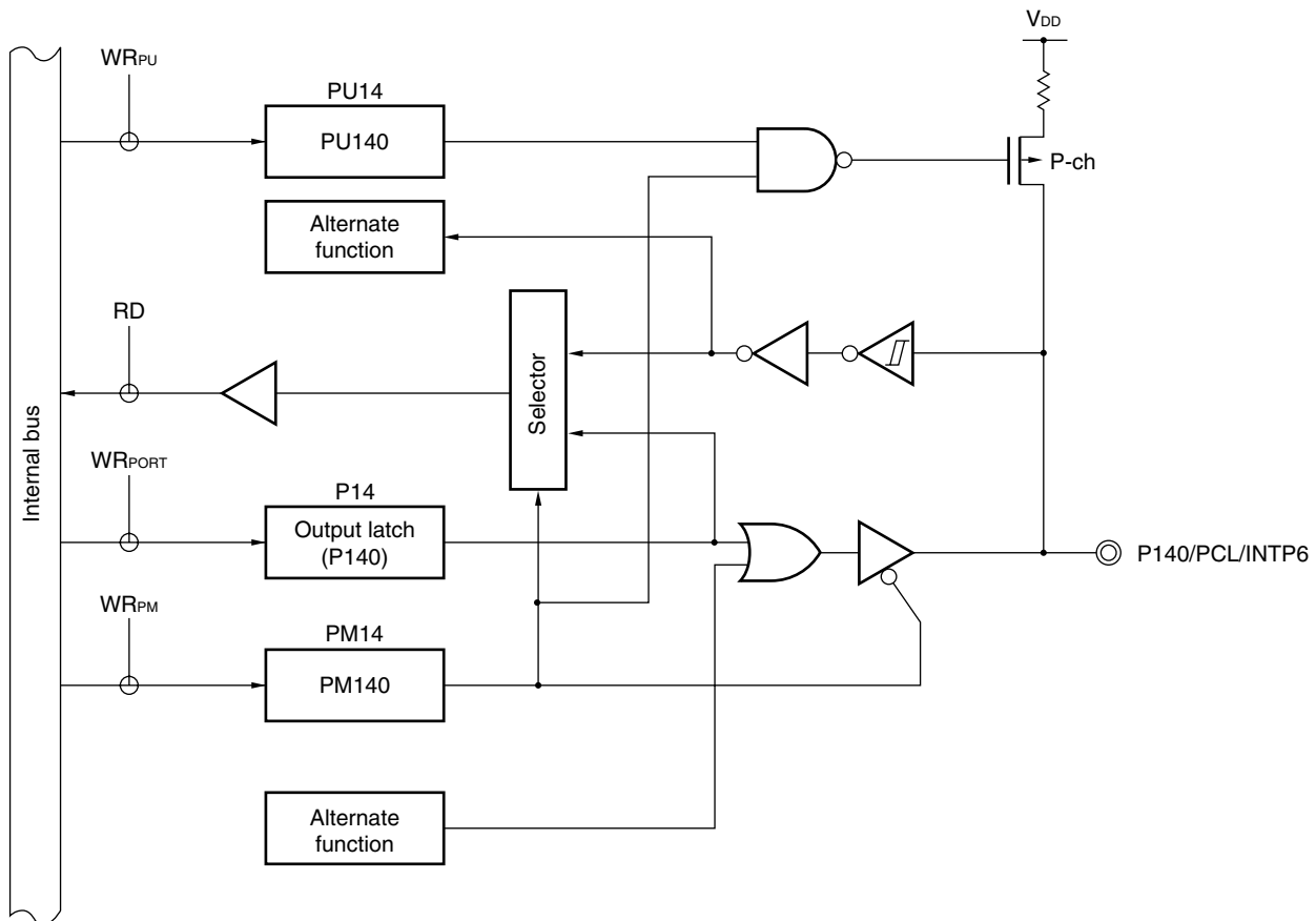
Figure 4-20. Block Diagram of P140 (48-Pin Products Only)
