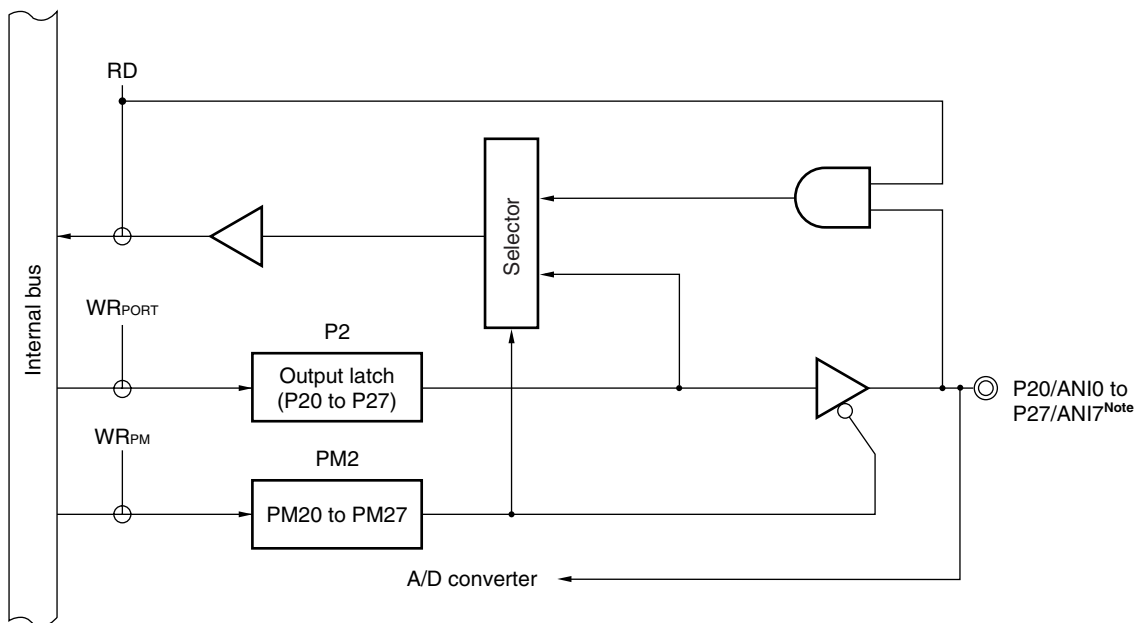
Figure 4-9. Block Diagram of P20 to P27
