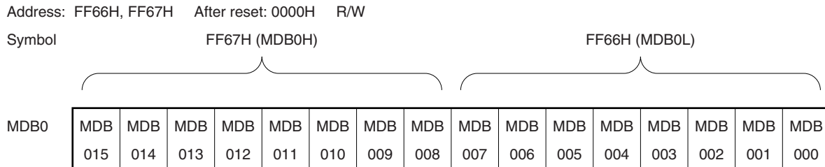
Figure 17-4. Format of Multiplication/Division Data Register B0 (MDB0)
