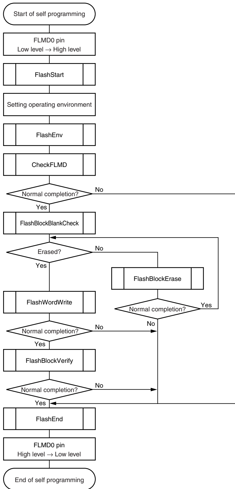
Figure 25-20. Flow of Self Programming (Rewriting Flash Memory)
