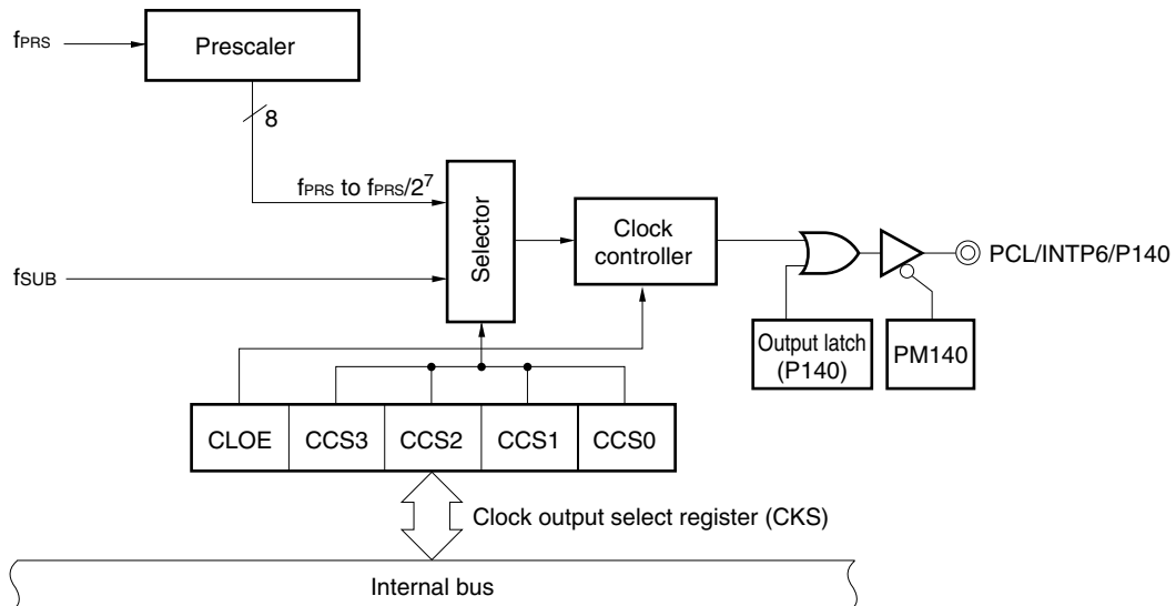
Figure 11-1. Block Diagram of Clock Output Controller
