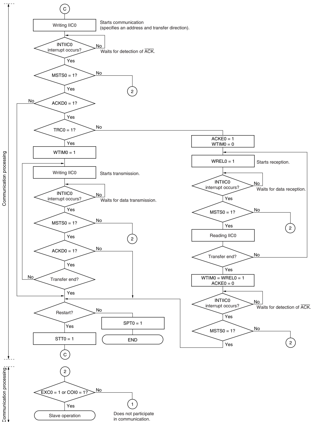
Figure 16-24. Master Operation in Multi-Master System (3/3)
