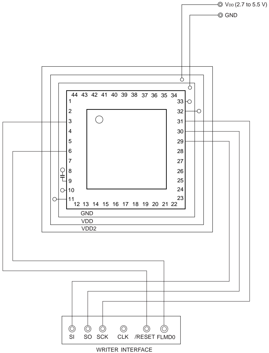
Figure 25-5. Example of Wiring Adapter for Flash Memory Writing in 3-Wire Serial I/O (CSI10) Mode (44-Pin Products)
