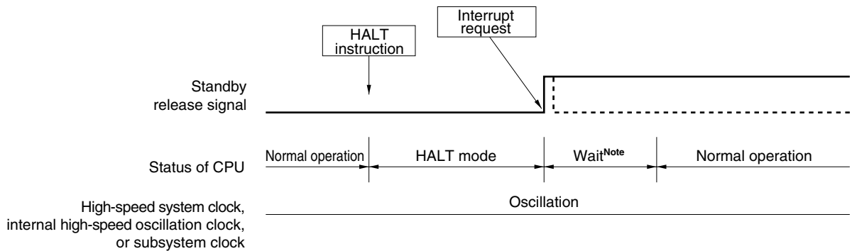
Figure 20-3. HALT Mode Release by Interrupt Request Generation
