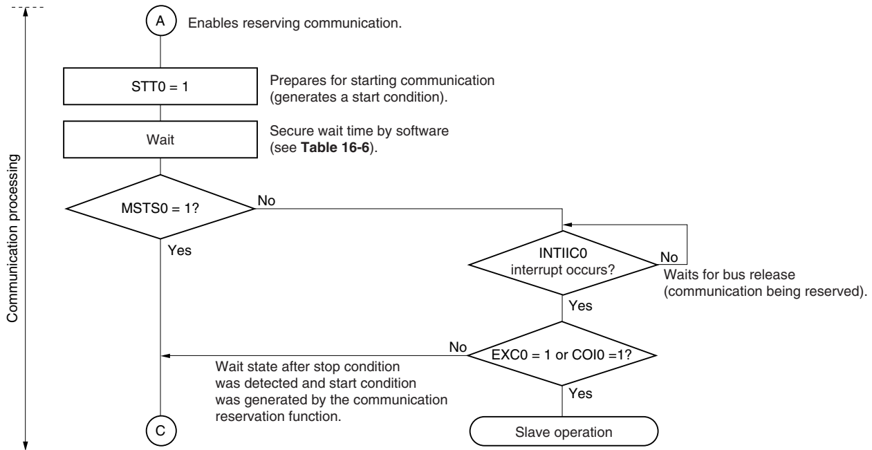
Figure 16-24. Master Operation in Multi-Master System (2/3)
