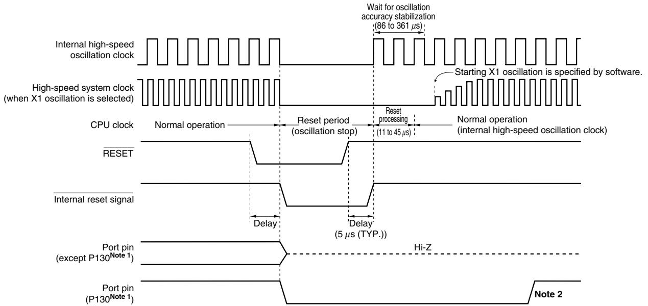
Figure 21-2. Timing of Reset by RESET Input
