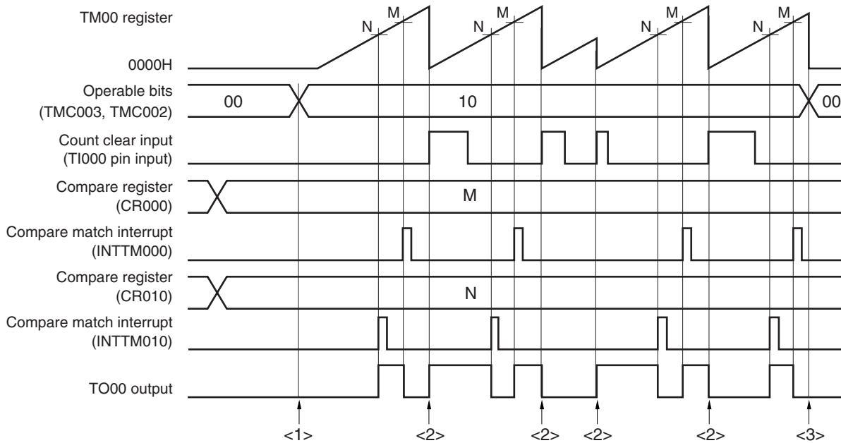
<R> Figure 6-31. Example of Software Processing in Clear & Start Mode Entered by TI000 Pin Valid Edge Input
