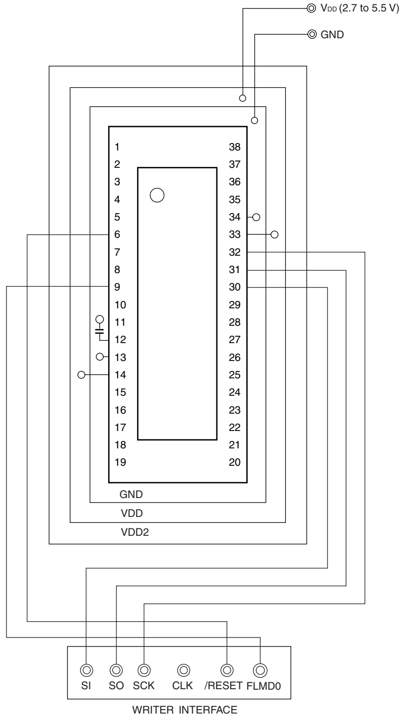
<R> Figure 25-3. Example of Wiring Adapter for Flash Memory Writing in 3-Wire Serial I/O (CS110) Mode (38-Pin Products)
