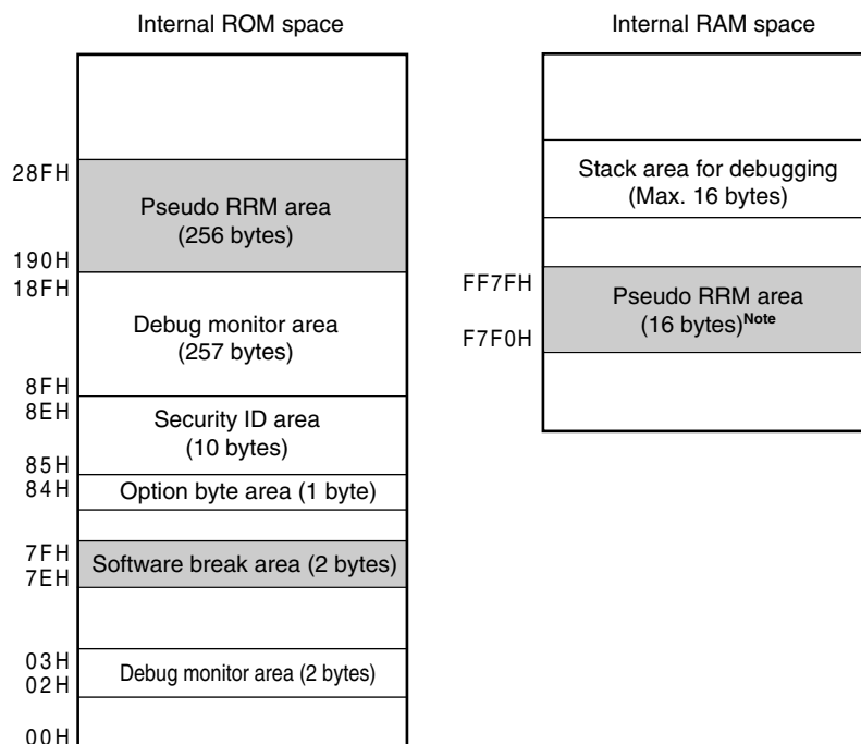
Figure 26-4. Reserved Area Used by QB-78K0MINI and QB-MINI2
