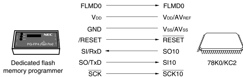
Figure 25-10. Communication with Dedicated Flash Memory Programmer (CSI10)
