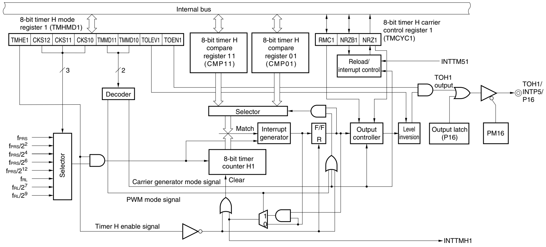
<R> Figure 8-2. Block Diagram of 8-bit Timer H1
