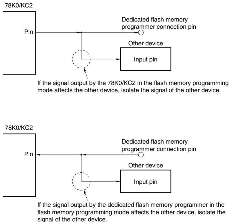
Figure 25-14. Malfunction of Other Device
