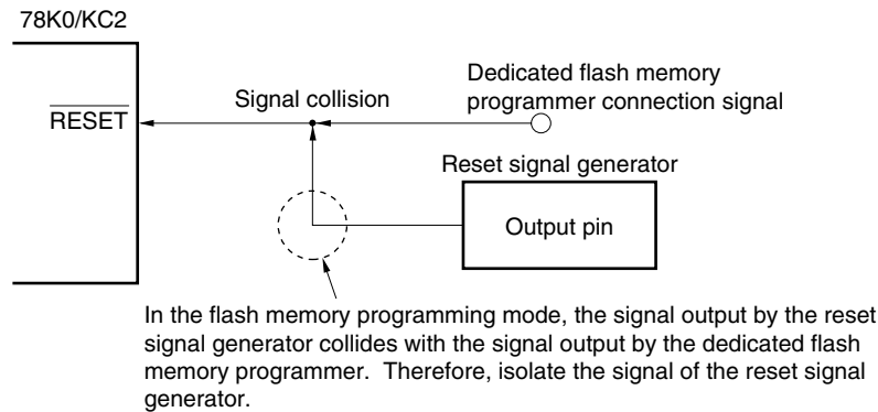
Figure 25-15. Signal Collision ( \overline{\text{RESET}} Pin)
