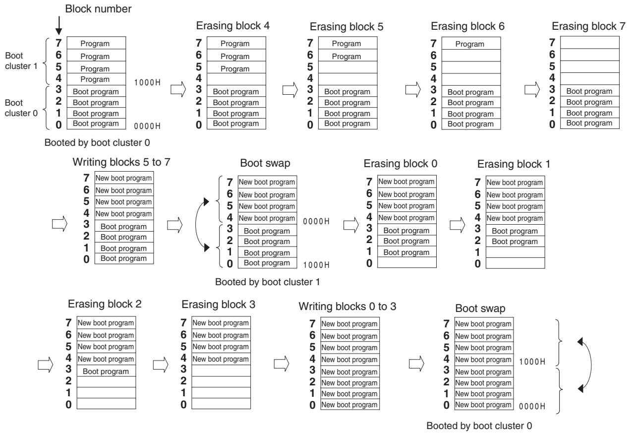
Figure 25-22. Example of Executing Boot Swapping
