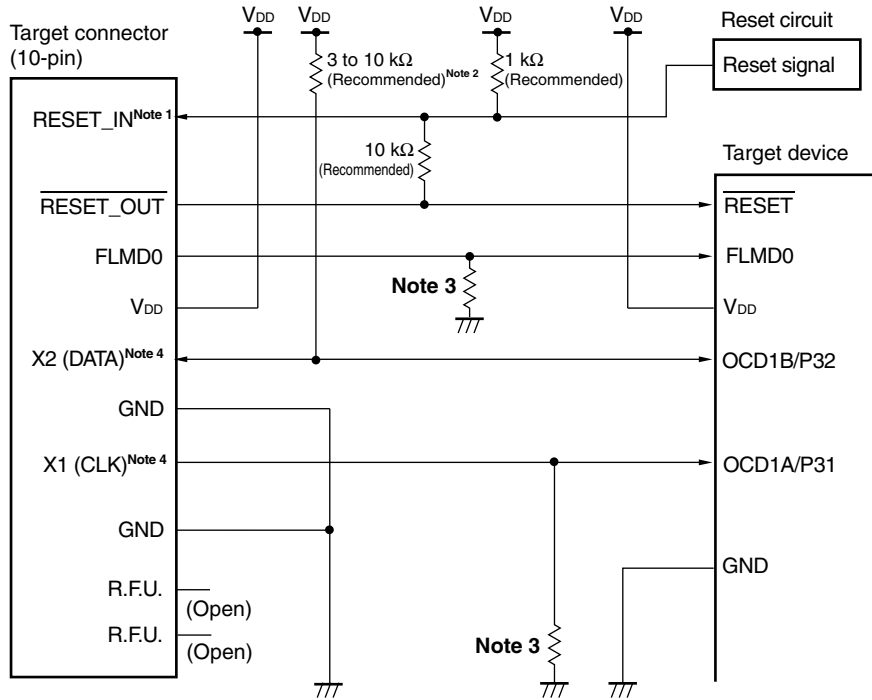
Figure 26-2. Connection Example of QB-78K0MINI or QB-MINI2 and \mu PD78F0513D, 78F0515D (When OCD1A/P31 and OCD1B/P32 Are Used)
