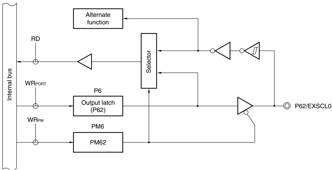
Figure 4-14. Block Diagram of P62
