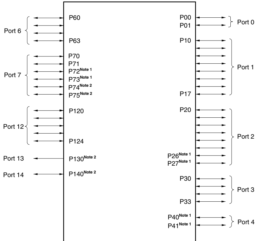
Figure 4-1. Port Types
