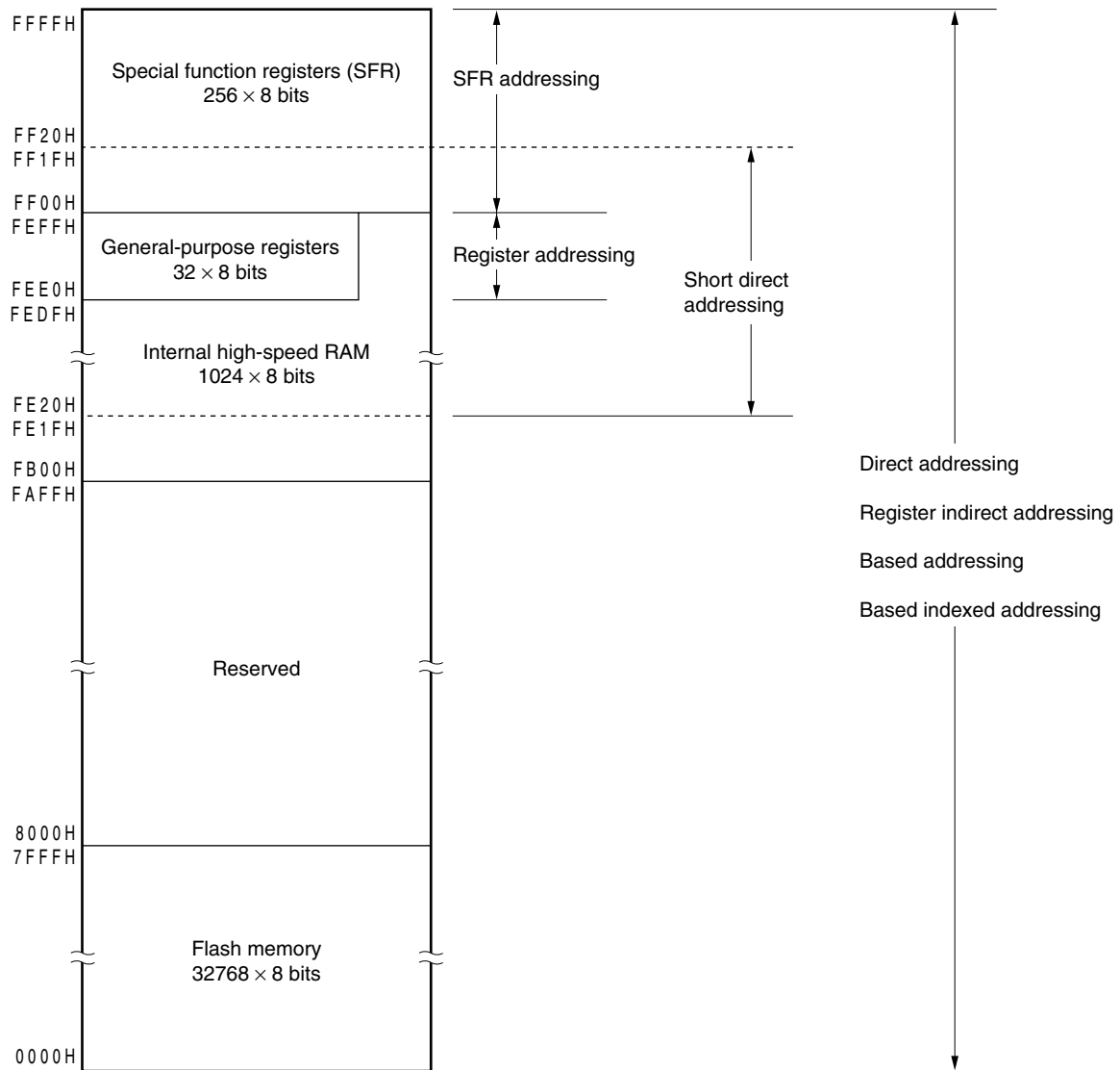
Figure 3-10. Correspondence Between Data Memory and Addressing ( \mu PD78F0513 and 78F0513D)
