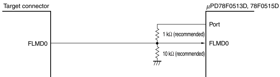
Figure 26-3. Connection of FLMD0 Pin for Self Programming by Means of On-Chip Debugging
