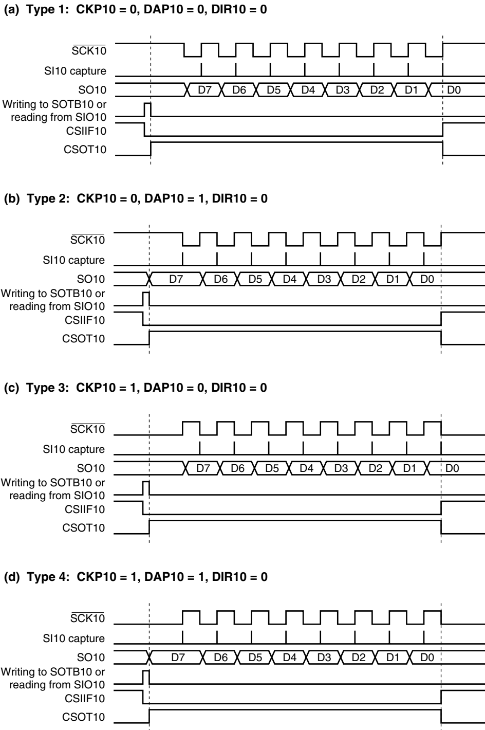
Figure 15-6. Timing of Clock/Data Phase
