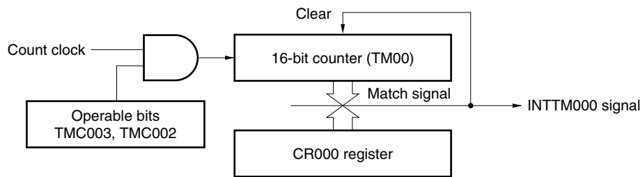
Figure 6-11. Block Diagram of Interval Timer Operation
