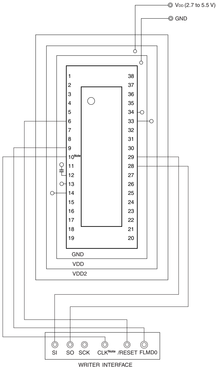
<R> Figure 25-4. Example of Wiring Adapter for Flash Memory Writing in UART (UART6) Mode (38-Pin Products)
