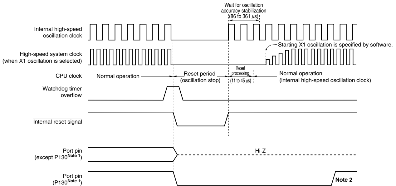
Figure 21-3. Timing of Reset Due to Watchdog Timer Overflow
