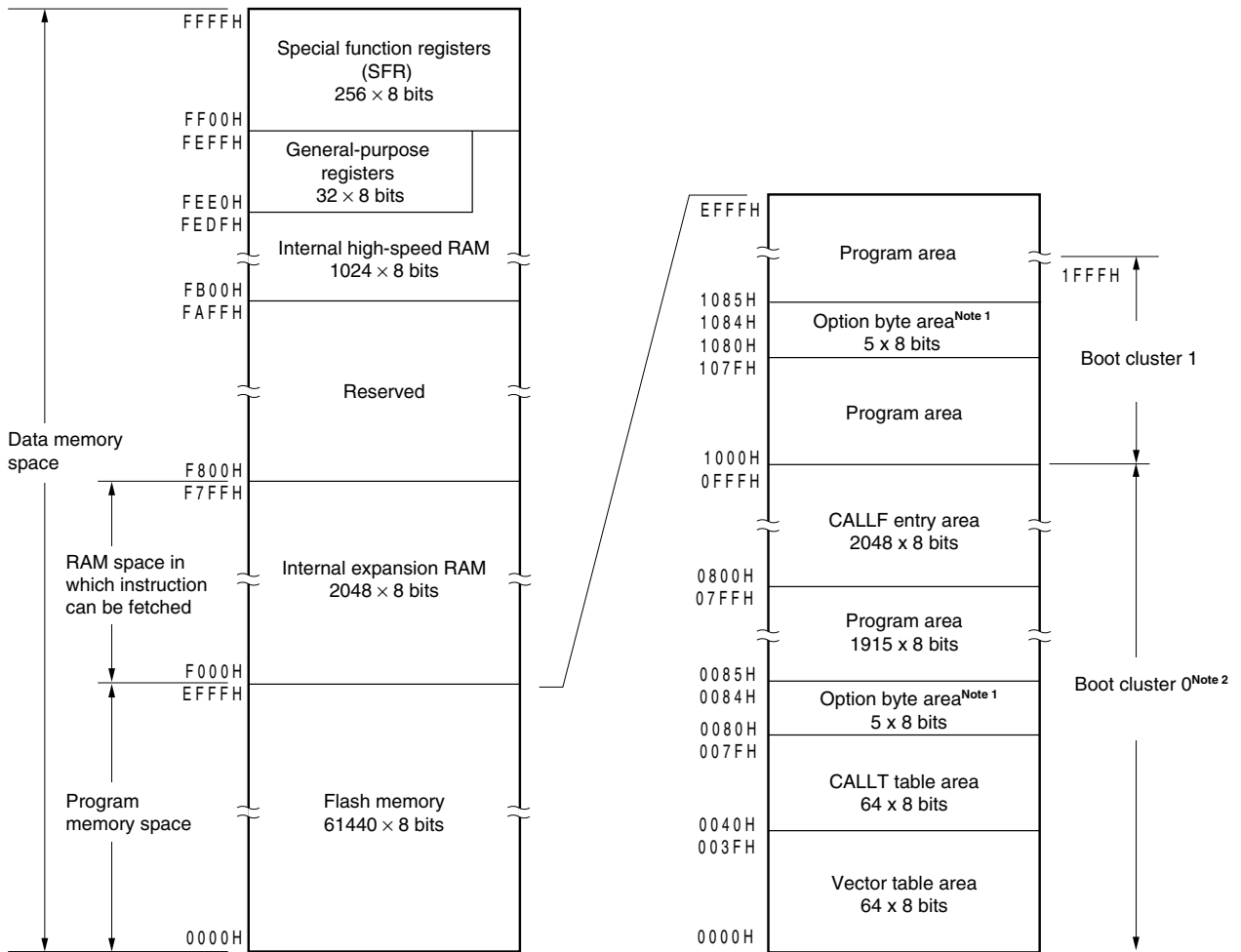
Figure 3-6. Memory Map ( \mu PD78F0515)
