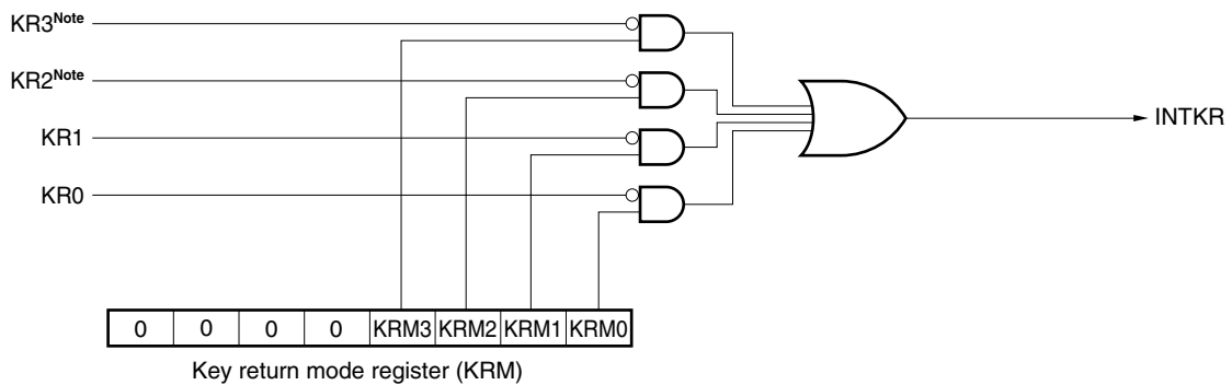
Figure 19-1. Block Diagram of Key Interrupt
