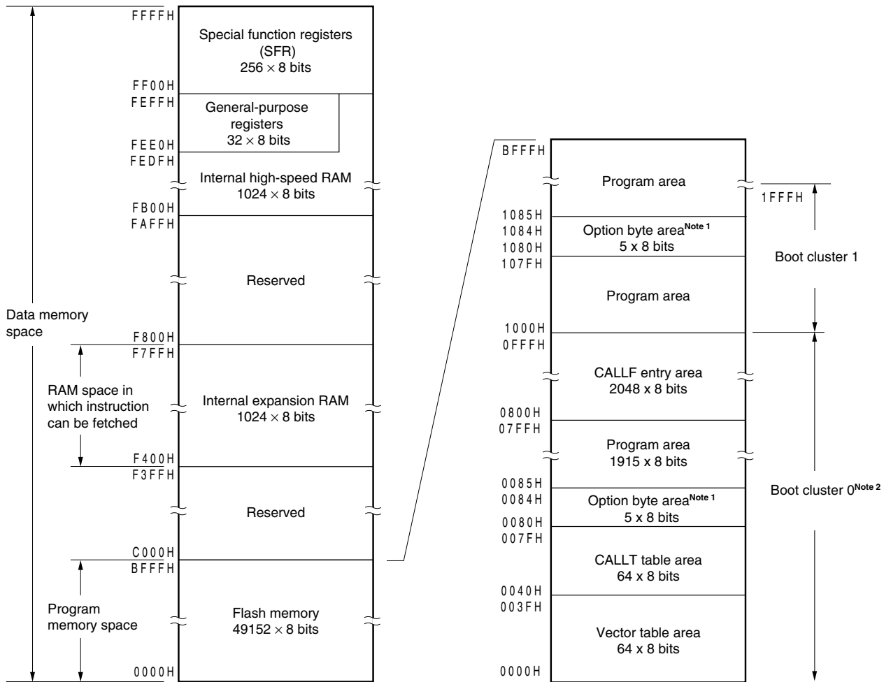
Figure 3-5. Memory Map ( \mu PD78F0514)
