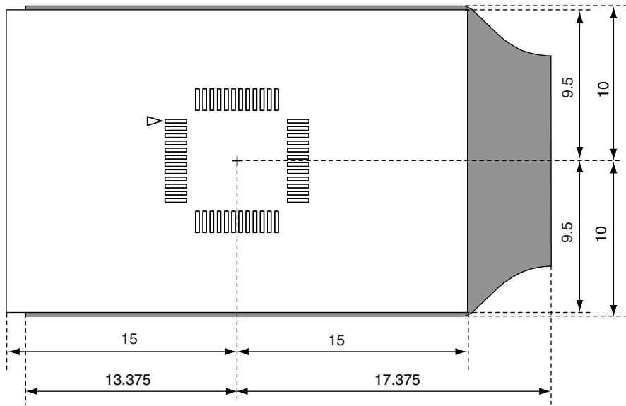
Figure B-2. For 48-Pin GA Package
