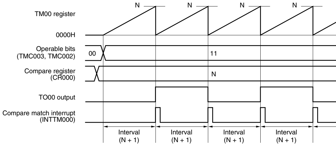
<R> Figure 6-16. Basic Timing Example of Square Wave Output Operation
