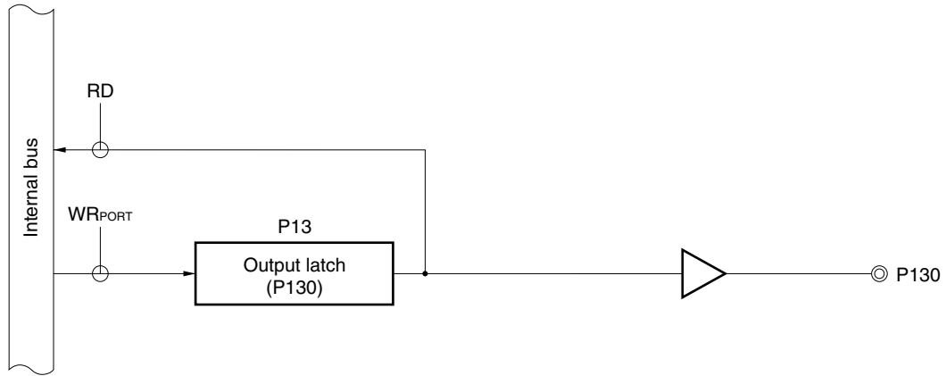
Figure 4-19. Block Diagram of P130 (48-Pin Products Only)
