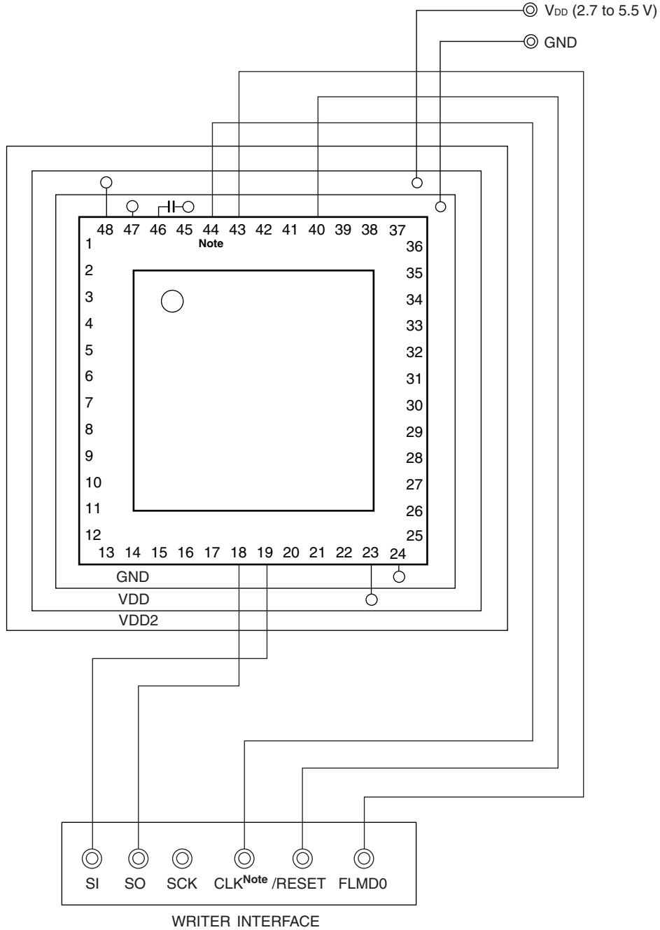
Figure 25-8. Example of Wiring Adapter for Flash Memory Writing in UART (UART6) Mode (48-Pin Products)
