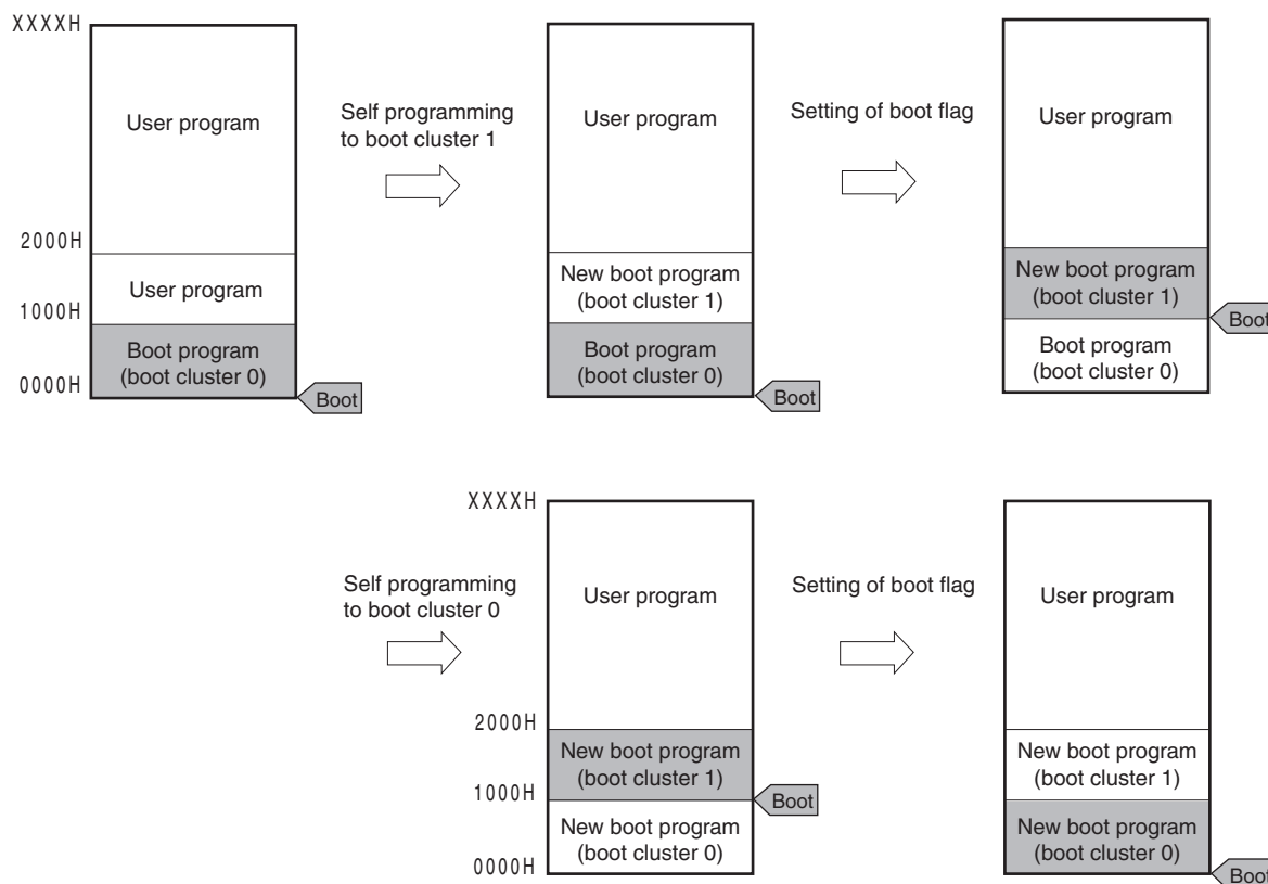
Figure 25-21. Boot Swap Function
