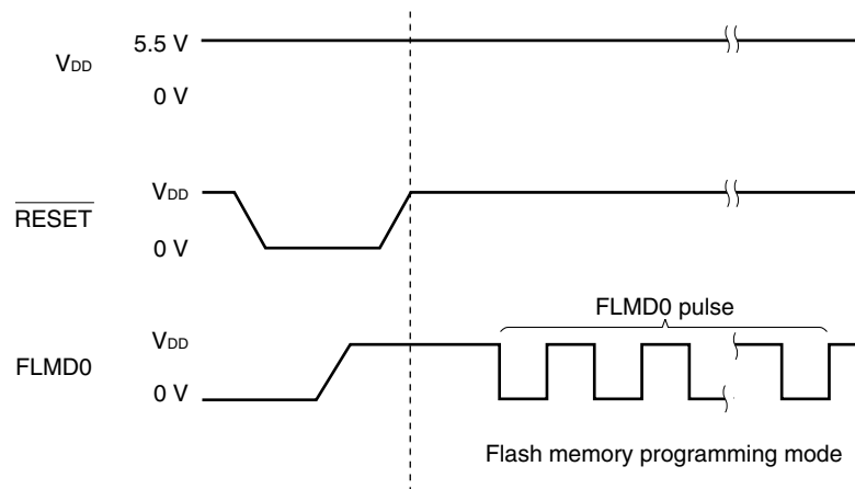
Figure 25-17. Flash Memory Programming Mode
