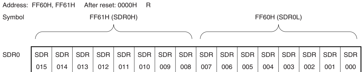
Figure 17-2. Format of Remainder Data Register 0 (SDR0)
