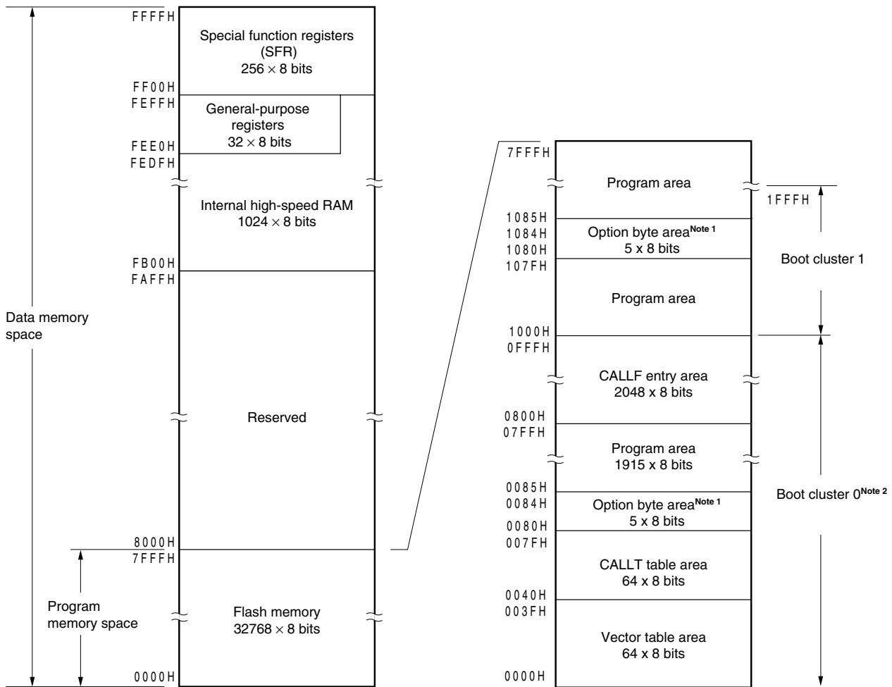
Figure 3-3. Memory Map (μPD78F0513)
