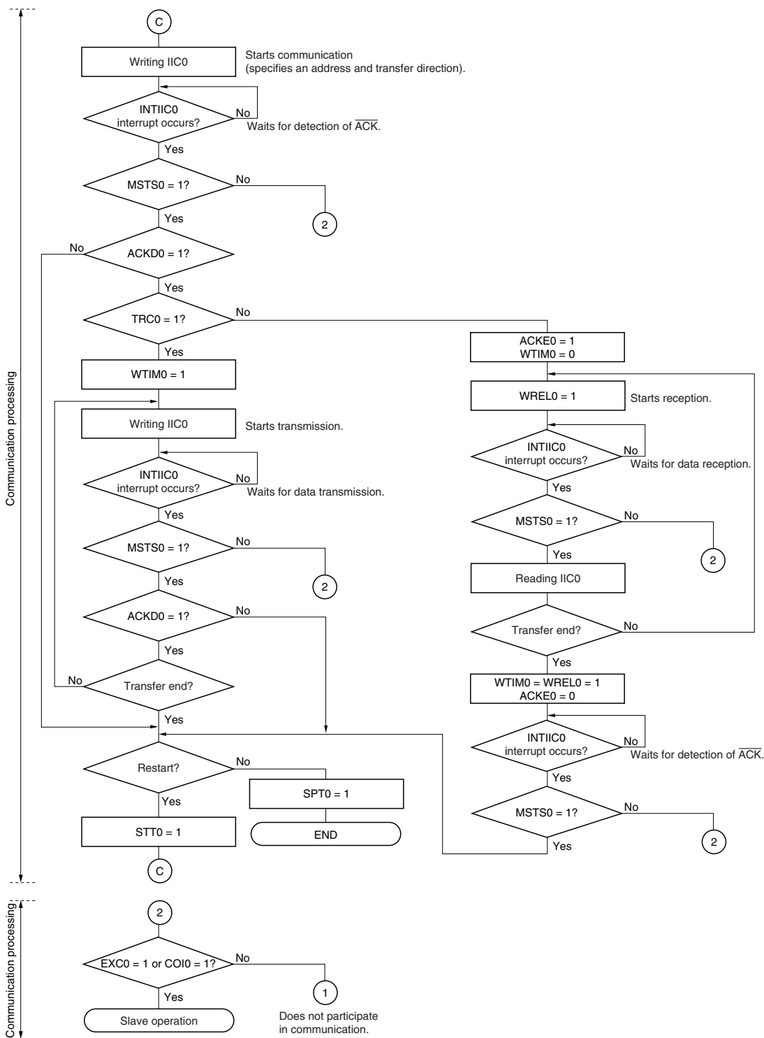
Figure 17-24. Master Operation Flowchart (Multi-Master System) (3/3)
