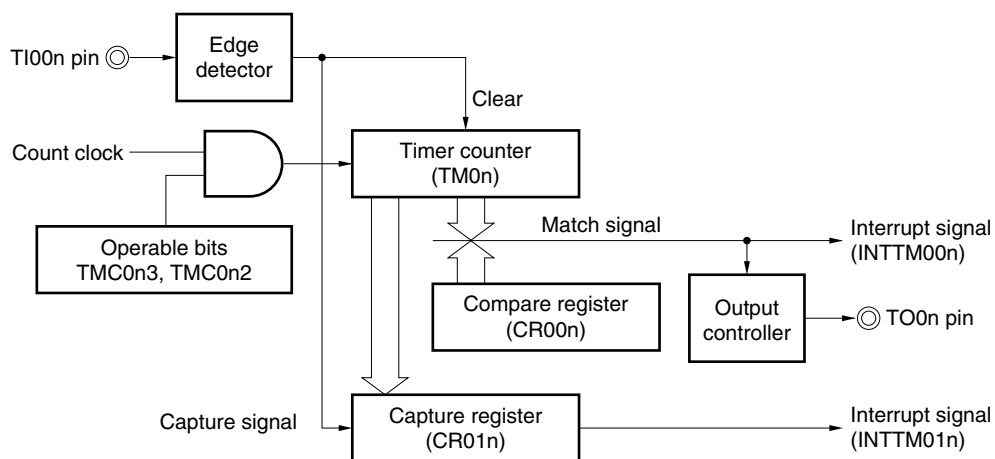
Figure 7-29. Block Diagram of Clear & Start Mode Entered by TI00n Pin Valid Edge Input (CR00n: Compare Register, CR01n: Capture Register)
