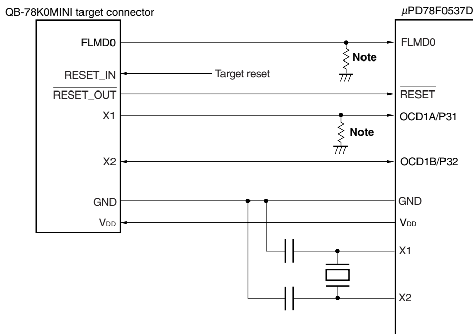
Figure 27-2. Connection Example of QB-78K0MINI and μPD78F0537D (When OCD1A and OCD1B Are Used)
