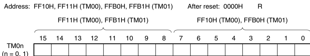
Figure 7-3. Format of 16-Bit Timer Counter 0n (TM0n)
