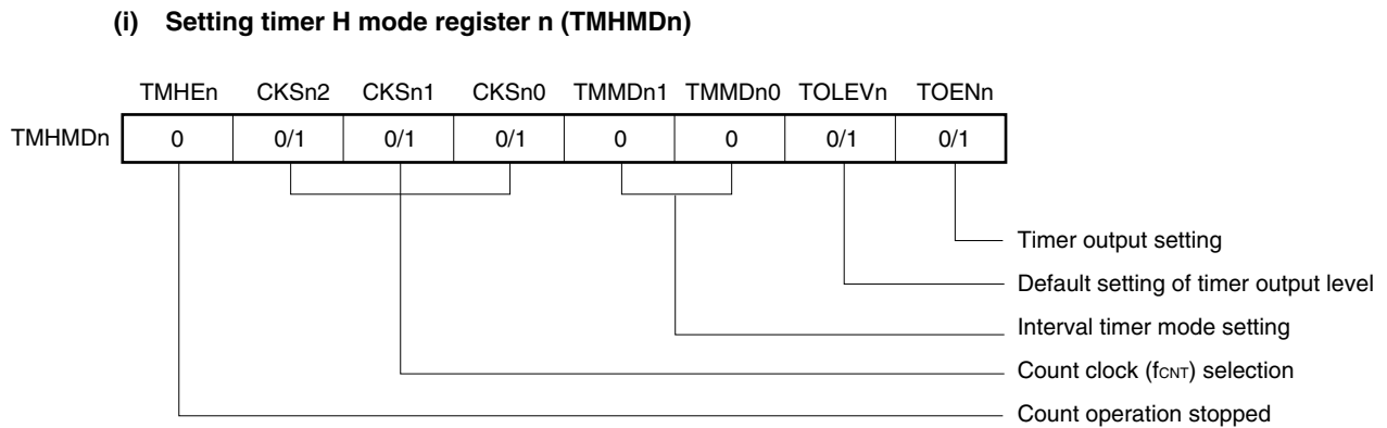
Figure 9-9. Register Setting During Interval Timer/Square-Wave Output Operation
