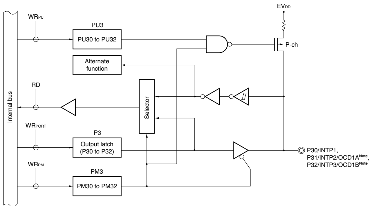
Figure 5-12. Block Diagram of P30 to P32
