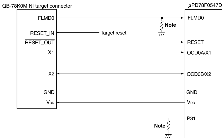
Figure 28-1. Connection Example of QB-78K0MINI and \mu PD78F0547D (When OCD0A/X1 and OCD0B/X2 Are Used)
