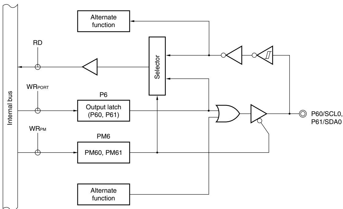
Figure 5-16. Block Diagram of P60 and P61
