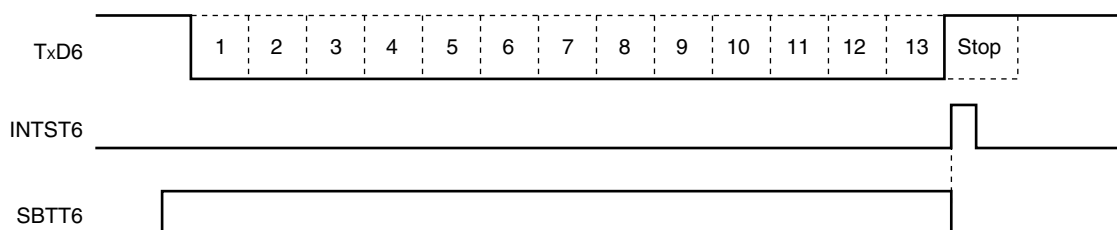
Figure 15-22. SBF Transmission
