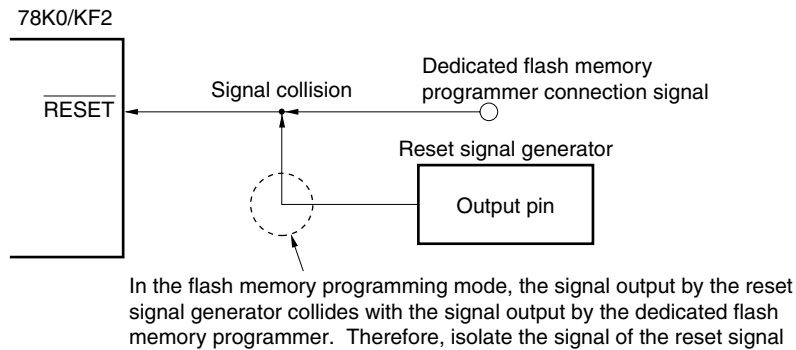
Figure 27-11. Signal Collision ( \overline{\text{RESET}} Pin)
