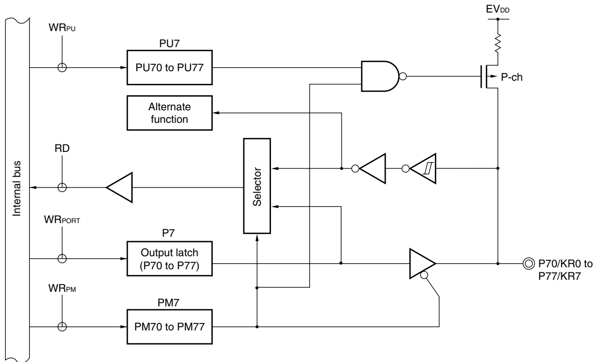
Figure 5-20. Block Diagram of P70 to P77
