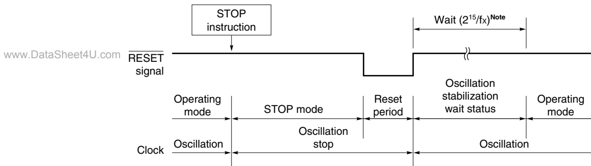
Figure 11-5. Releasing STOP Mode by \overline{\text{RESET}} Input
