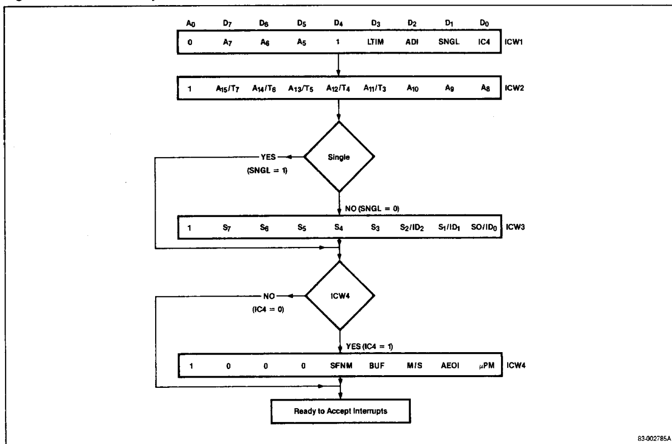
Figure 1. Initialization Sequence
