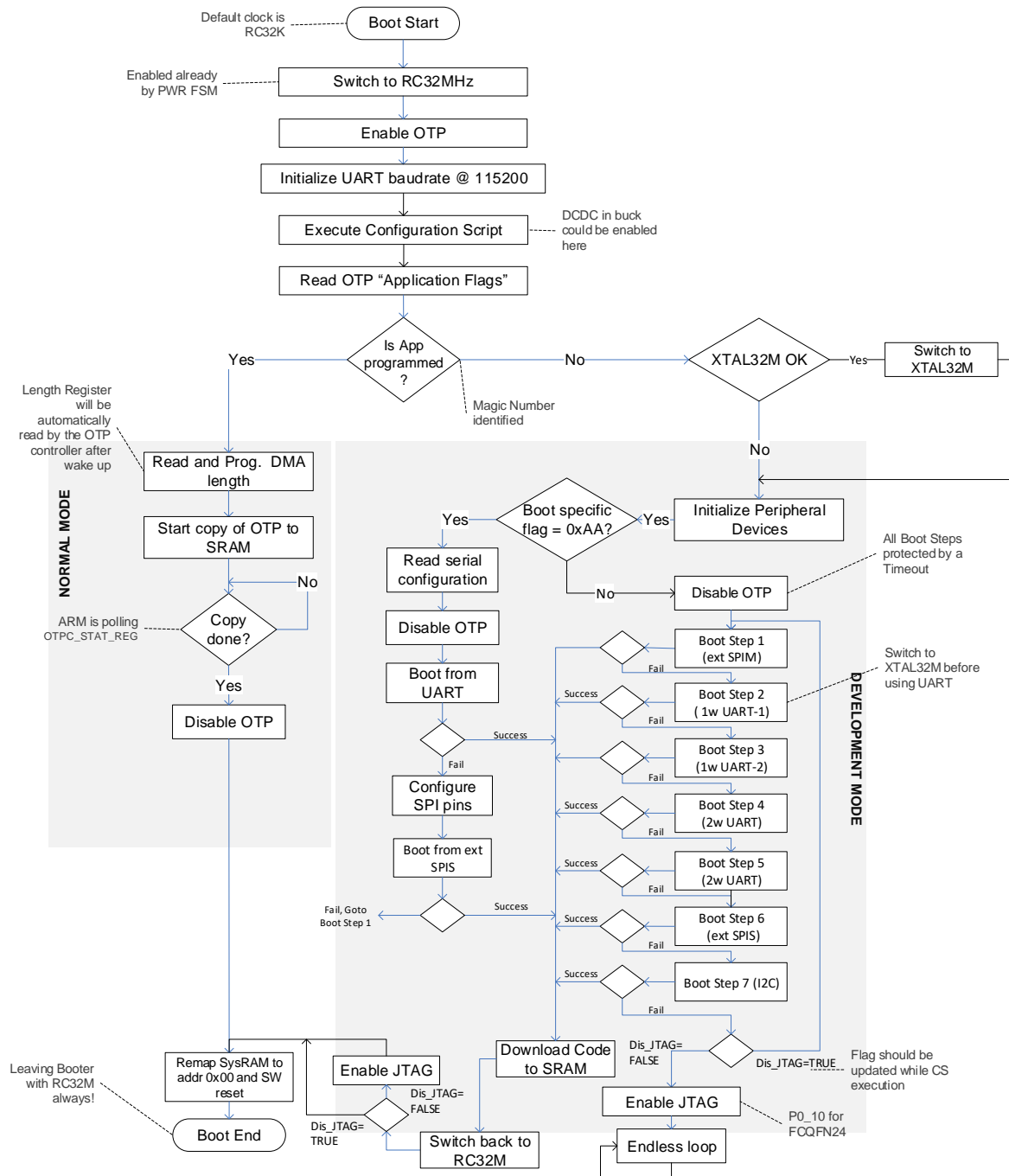
Figure 12. BootROM sequence
