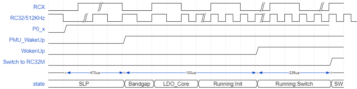
Figure 9. Wake-up (Buck)
