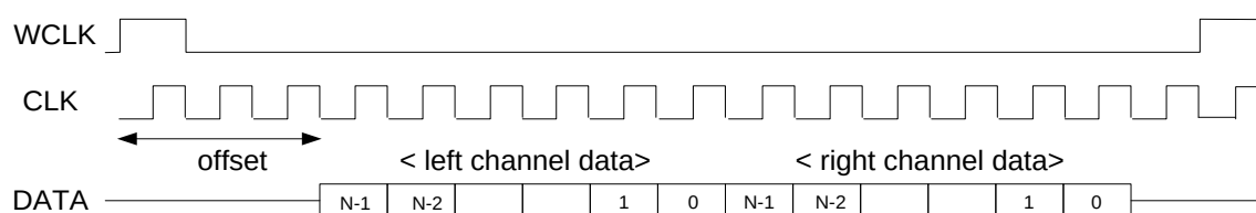
Figure 39: TDM DSP format
