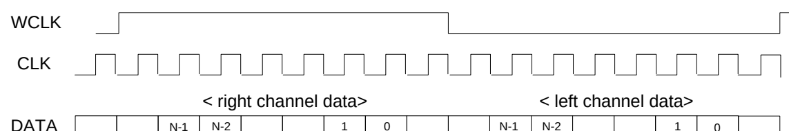
Figure 36: I2S format
