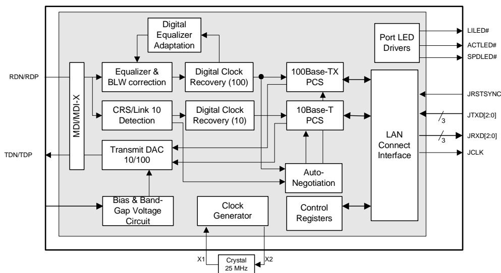
Figure 1. 82562EX Block Diagram
