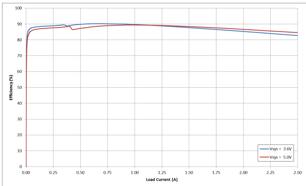
Figure 9: BUCKCORE2 Efficiency in AUTO Mode, V_{OUT} = 1.2\text{ V}
