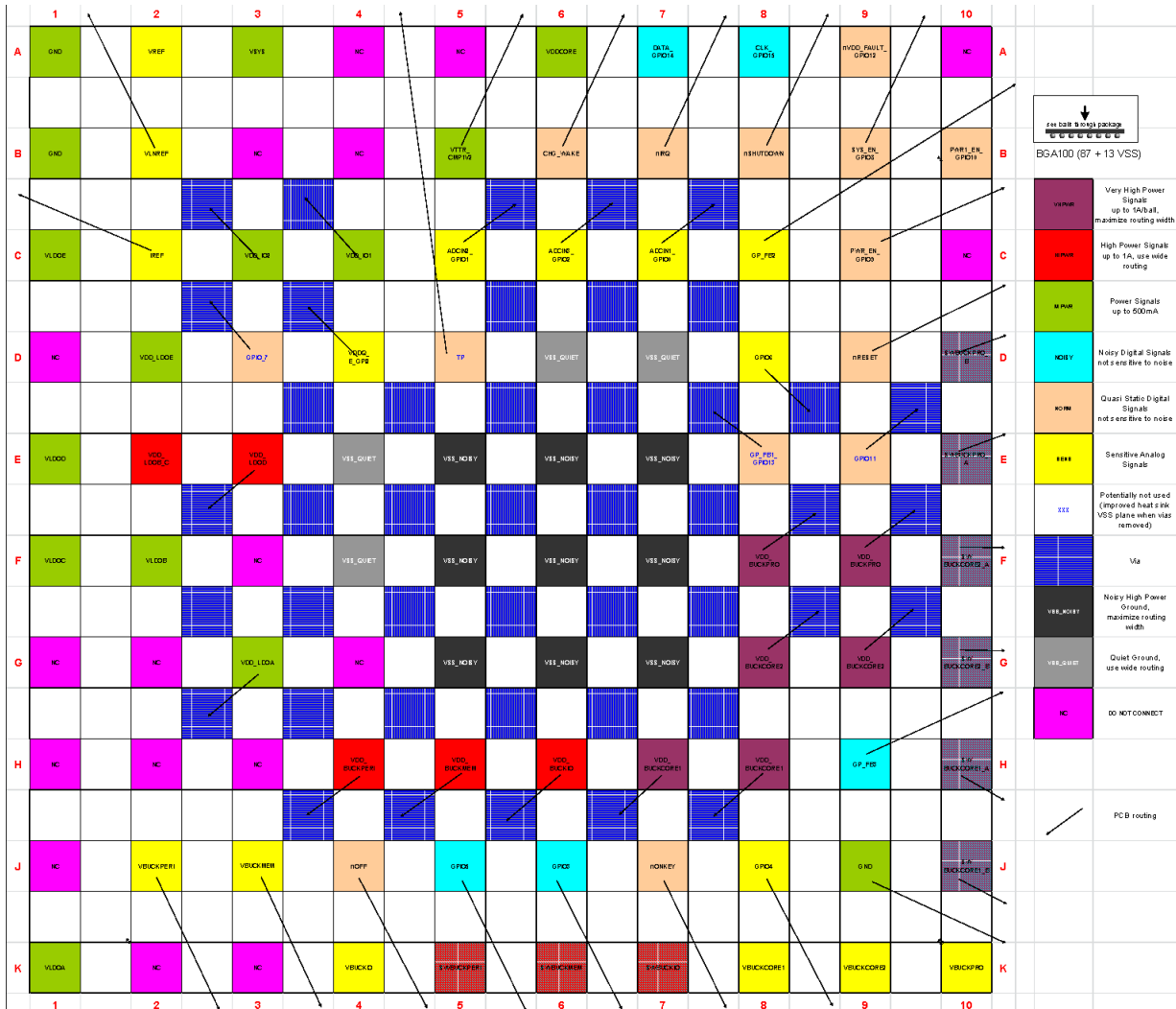
Figure 4: Connection Diagram
