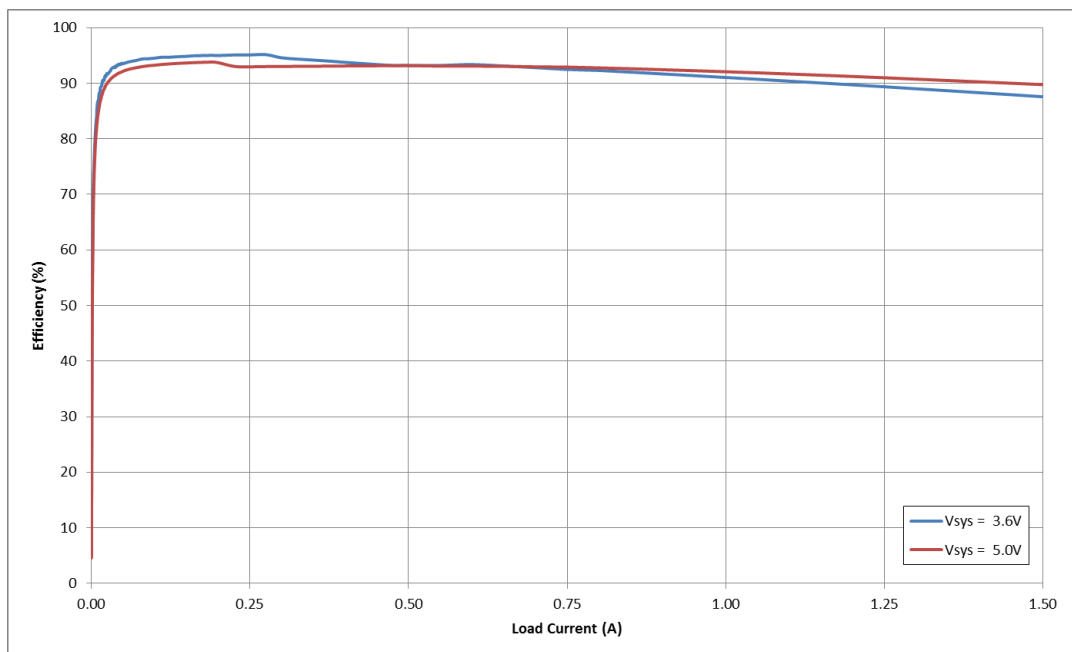
Figure 13: BUCKPERI Efficiency in AUTO Mode, V_{OUT} = 2.86\text{ V}
