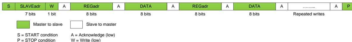
Figure 24: Repeated Write (DATA Line)
