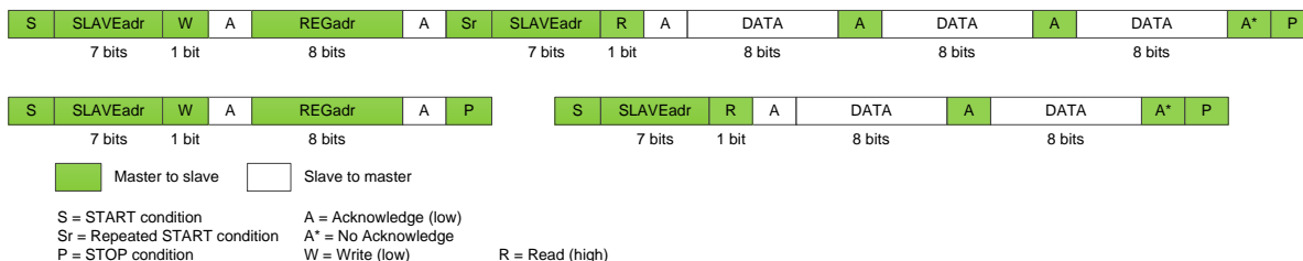
Figure 22: Examples of Page Read (DATA Line)
