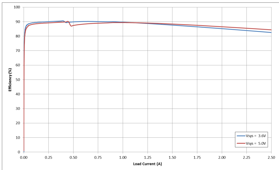
Figure 8: BUCKCORE1 Efficiency in AUTO Mode, V_{OUT} = 1.2\text{ V}
