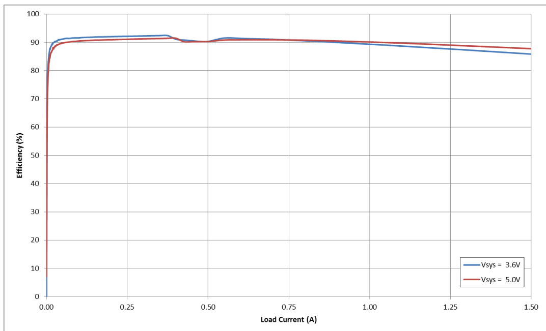
Figure 12: BUCKIO Efficiency in AUTO Mode, V_{OUT} = 1.8\text{ V}
