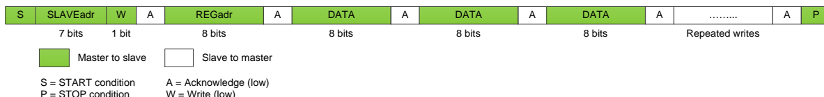
Figure 23: Page Write (DATA Line)
