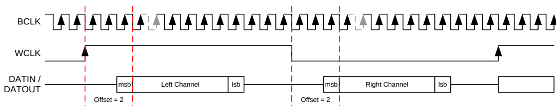
Figure 58: TDM Left Justified Format
