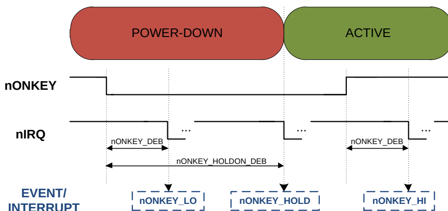
Figure 13: nONKEY ON
