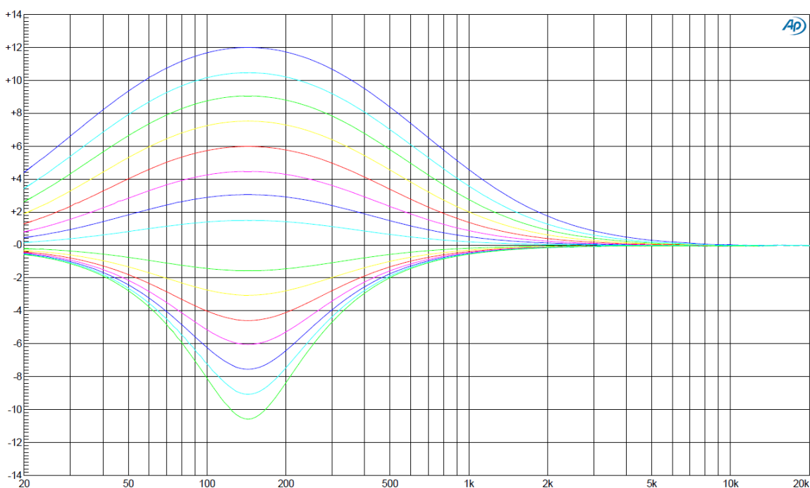
Figure 39: DAC Equalizer Filter Band 2 Frequency Response at FS = 48 kHz
