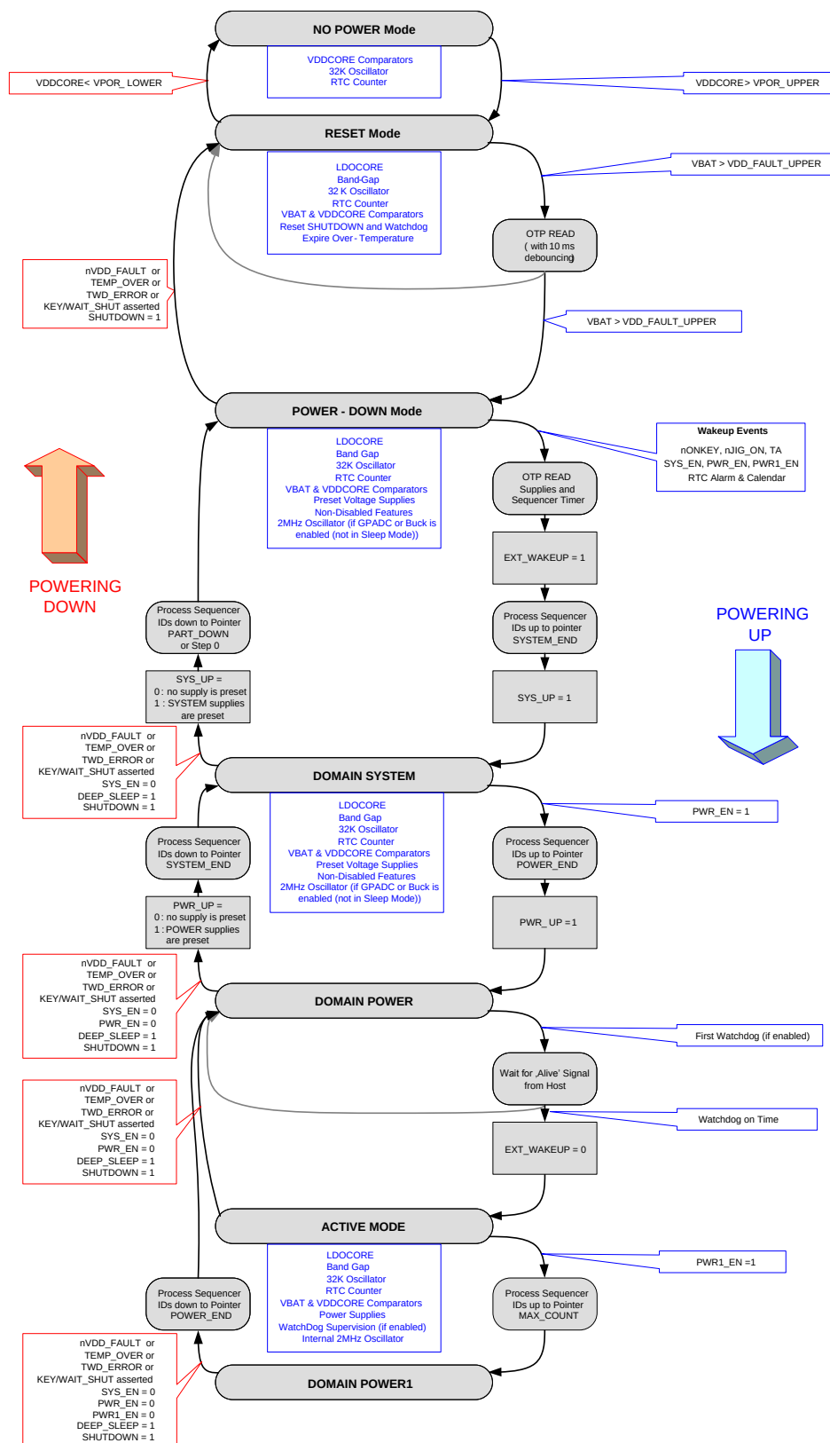
Figure 12: Operating Modes
