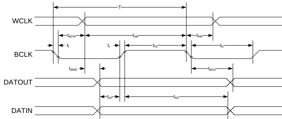
Figure 25: Digital Audio Interface Timing Diagram
