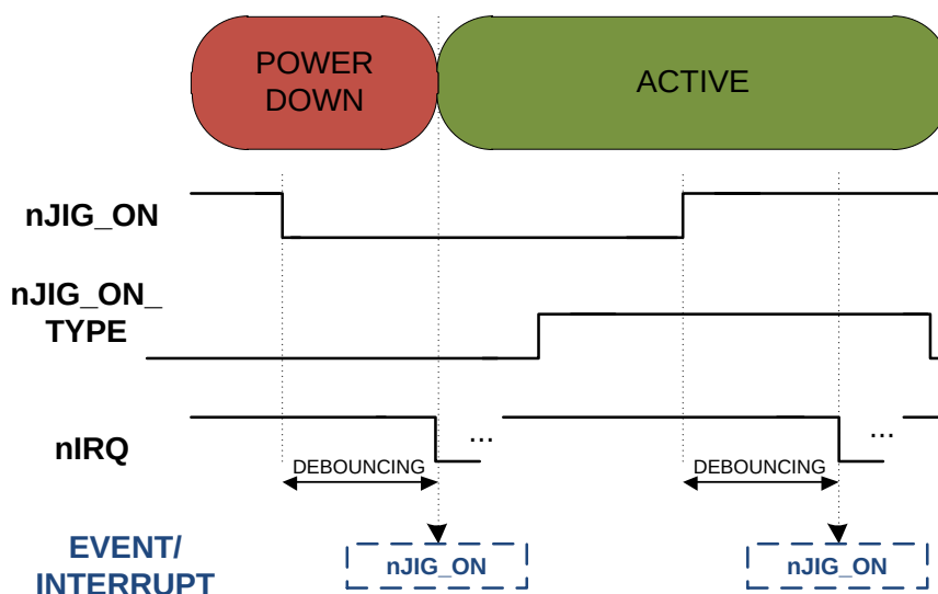
Figure 14: nJIG_ON ON
