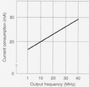
Output frequency vs. current consumption
