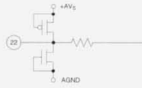
Reference Pins ( V_{REF} , I_{REF} , VG)
