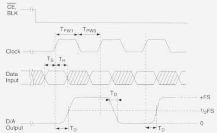
Timing Diagram
