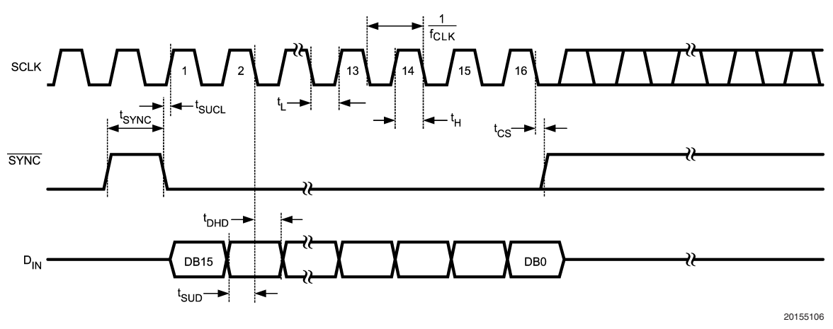
FIGURE 2. DAC081S101 Timing
