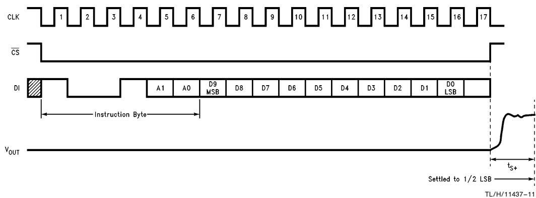
FIGURE 1. Write to One DAC with Update of Output ( \overline{A\bar{U}} = 1 ), 10 MHz Maximum CLK Rate
