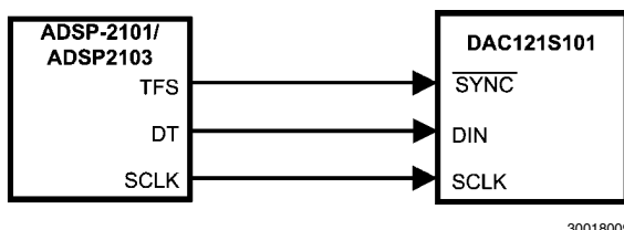
FIGURE 5. ADSP-2101/2103 Interface
