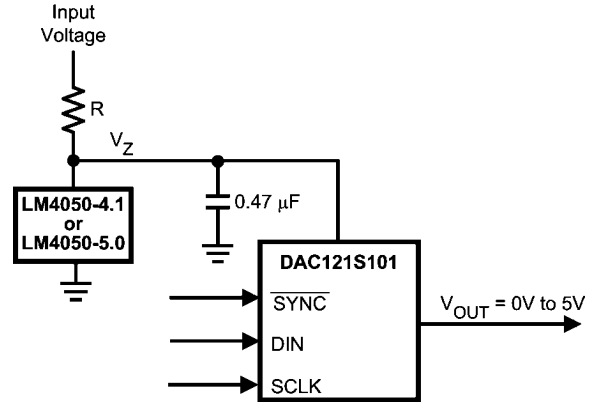
FIGURE 10. The LM4050 as a power supply
