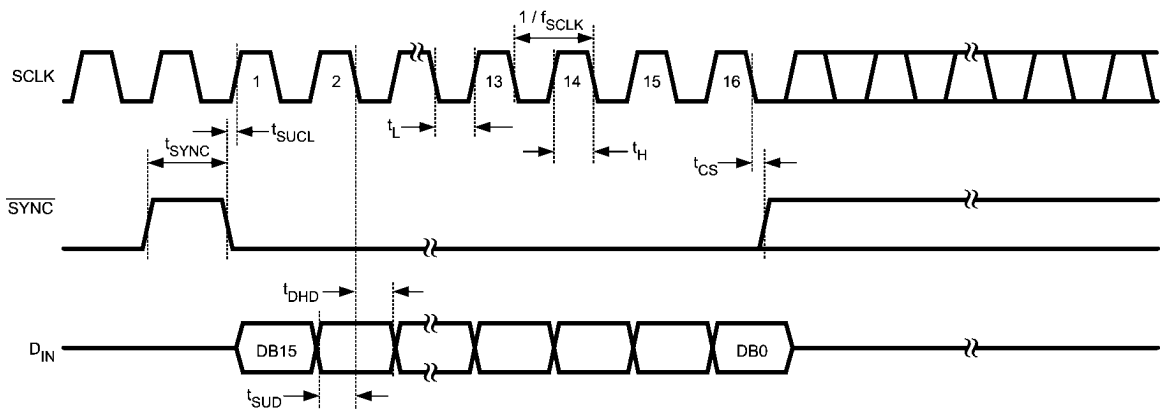
FIGURE 2. DAC121S101 Timing
