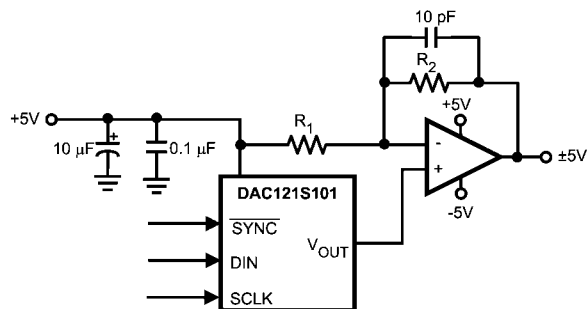
FIGURE 13. Bipolar Operation
