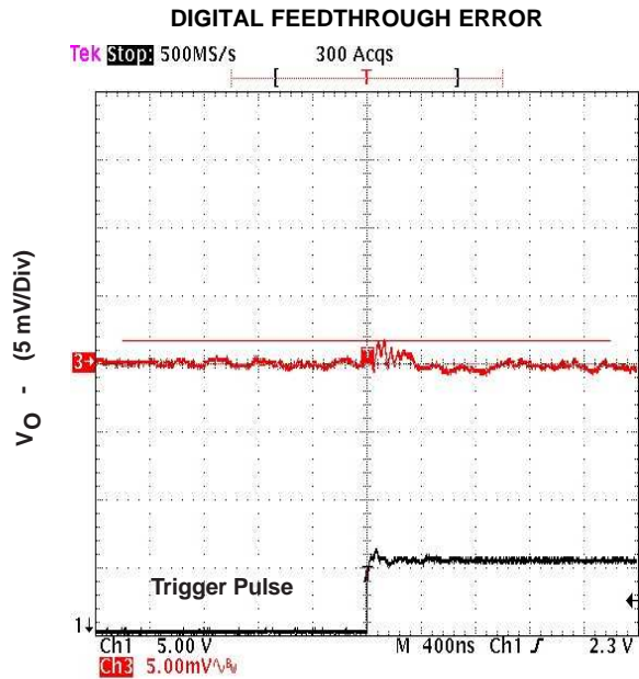
Time - (400 nS/Div)
