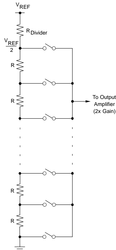
Figure 48. Resistor String
