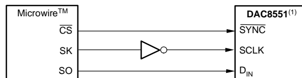
Figure 53. DAC8551 to Microwire Interface
