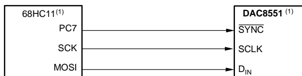
Figure 54. DAC8551 to 68HC11 Interface
