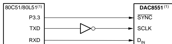
Figure 52. DAC8551 to 80C51/80L51 Interface
