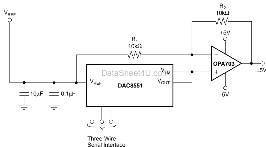
Figure 56. Bipolar Output Range
