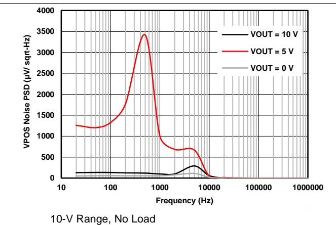
Figure 86. VPOS Noise Density (VOUT Mode) vs Frequency
