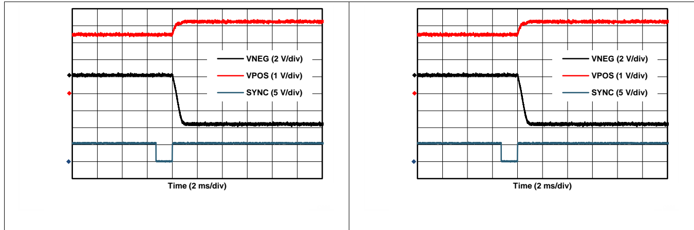
Figure 83. Buck-Boost Converter Power-On (IOUT Mode)
