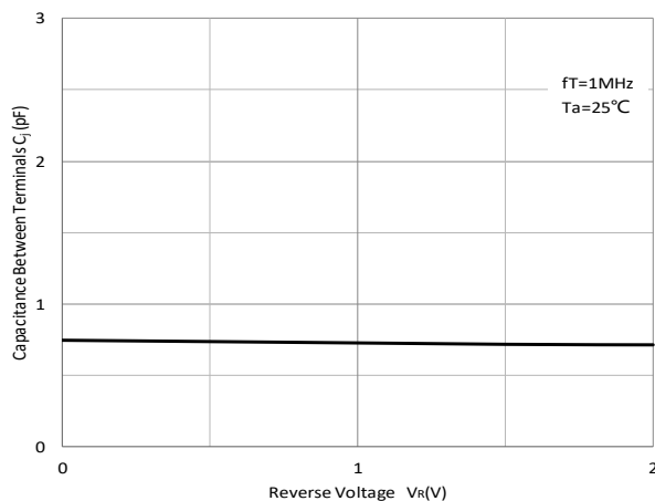
Fig 2: Capacitance Capability
