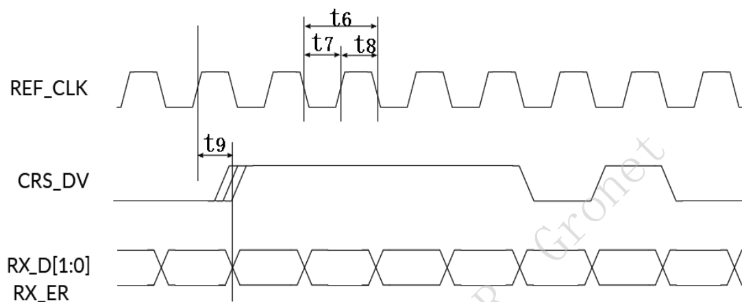
Figure 5. RMII Receive Timing
