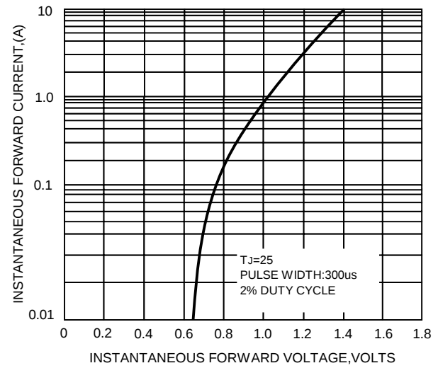
FIG.4-TYPICAL FORWARD CHARACTERISTICS
