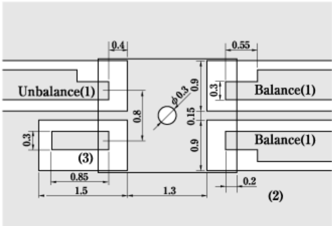
Land Pattern
