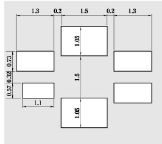
Resist Pattern
