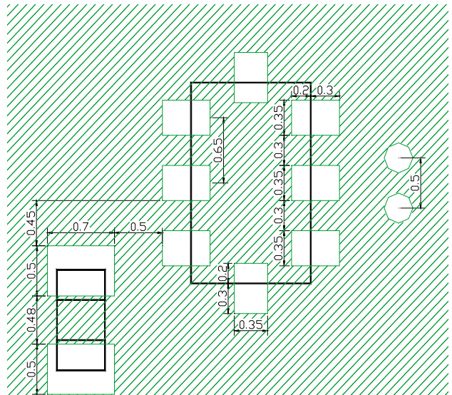
Resist Pattern
