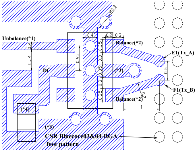
Land Pattern
