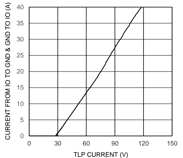
Figure 8. TLP Curve ( t_p = 100\text{ns} )
