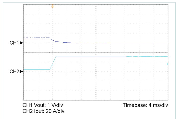
Figure 8 — 10% to 100% load transient response, V_{IN} = 275\text{ V} , nominal trim, C_{OUT\_EXT} = 1000\text{ }\mu\text{F}
