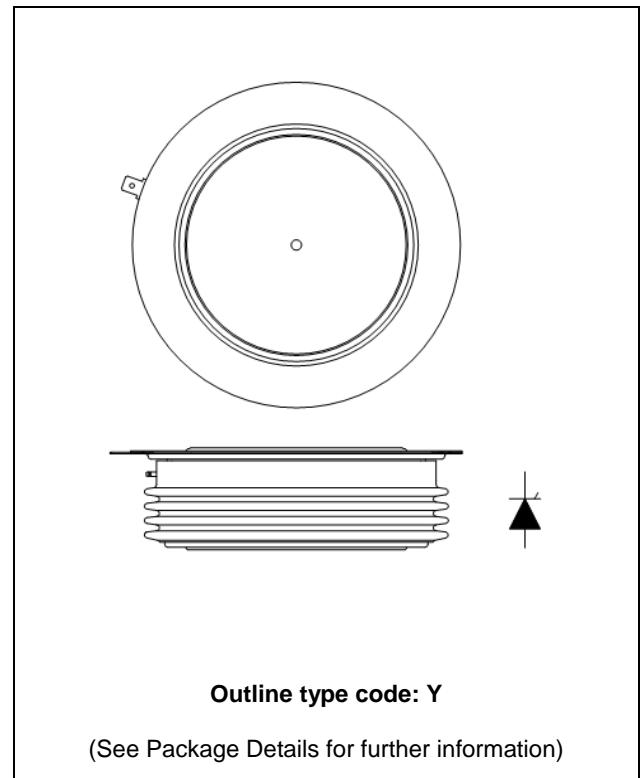
Fig. 1 Package outline
