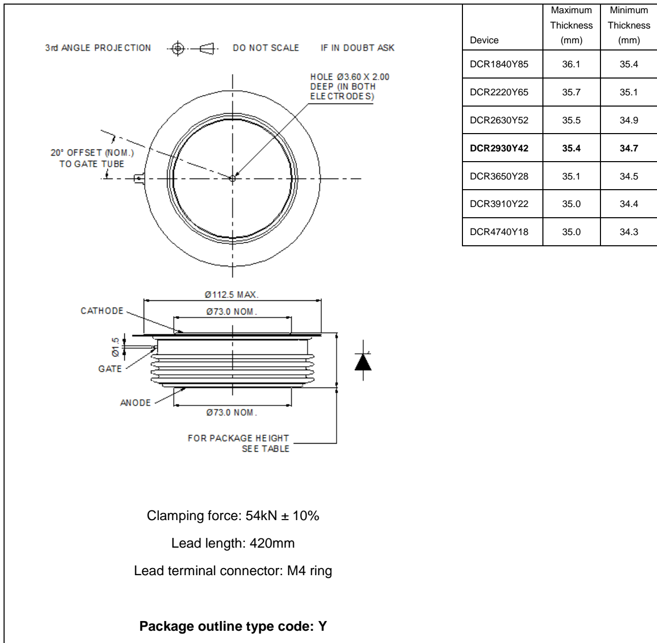
Fig. 16 Package outline
