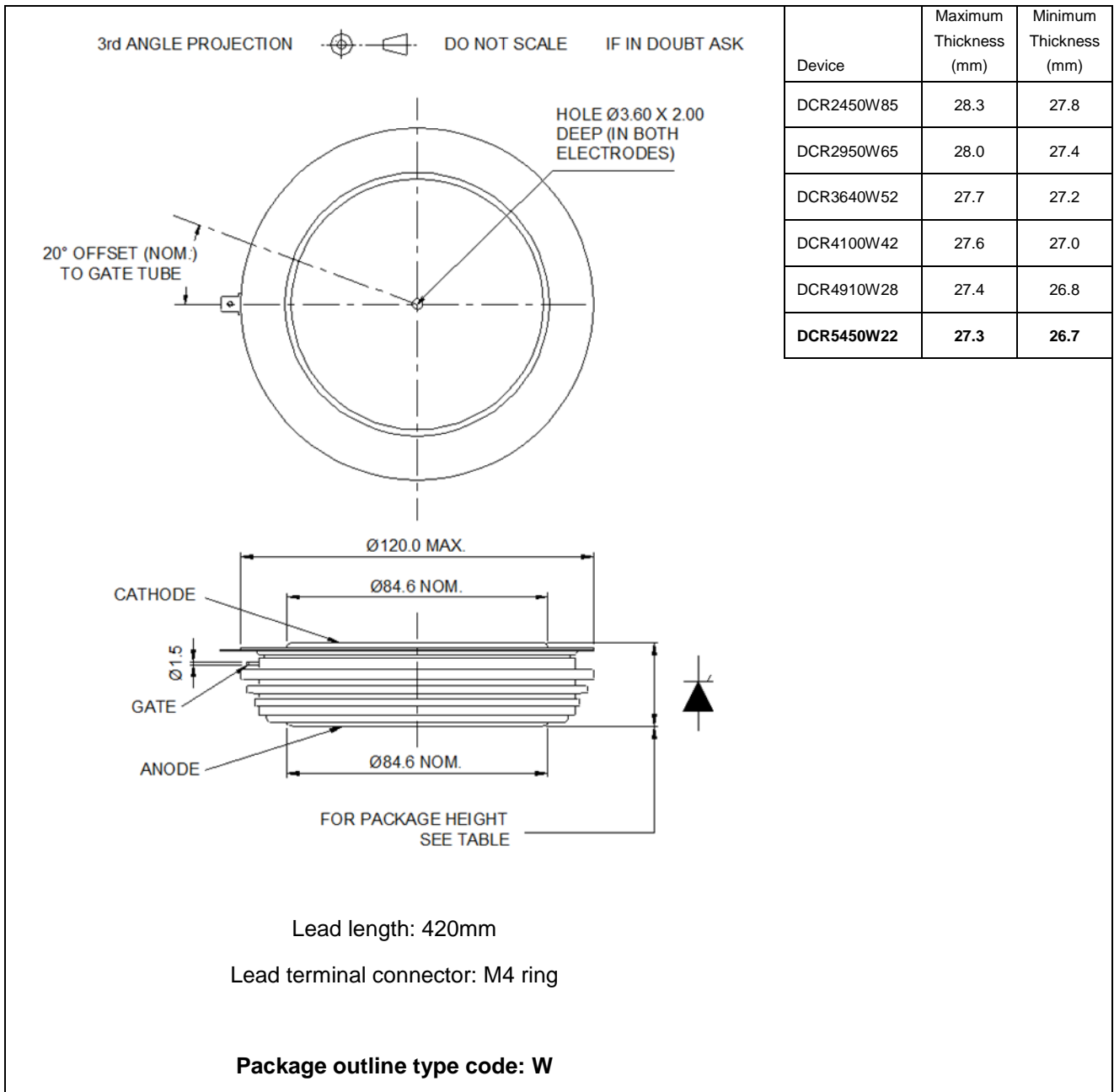
Fig. 16 Package outline
