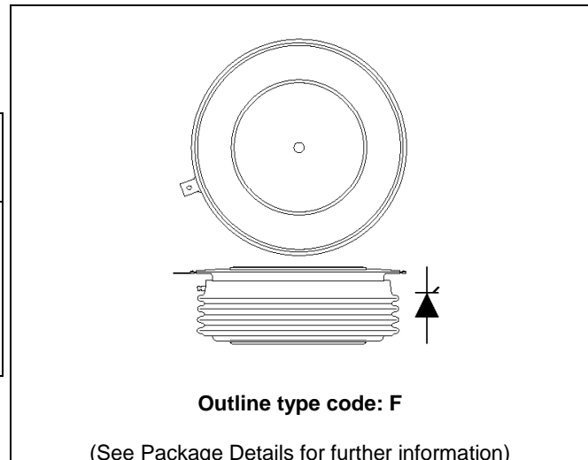
Fig. 1 Package outline
