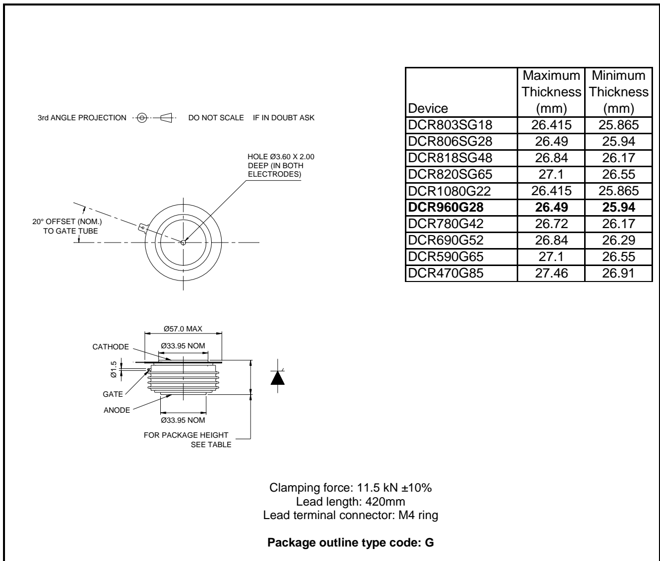
Fig.14 Package outline
