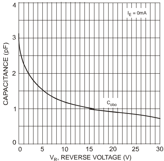
Fig. 21 Typical Capacitance Characteristics
