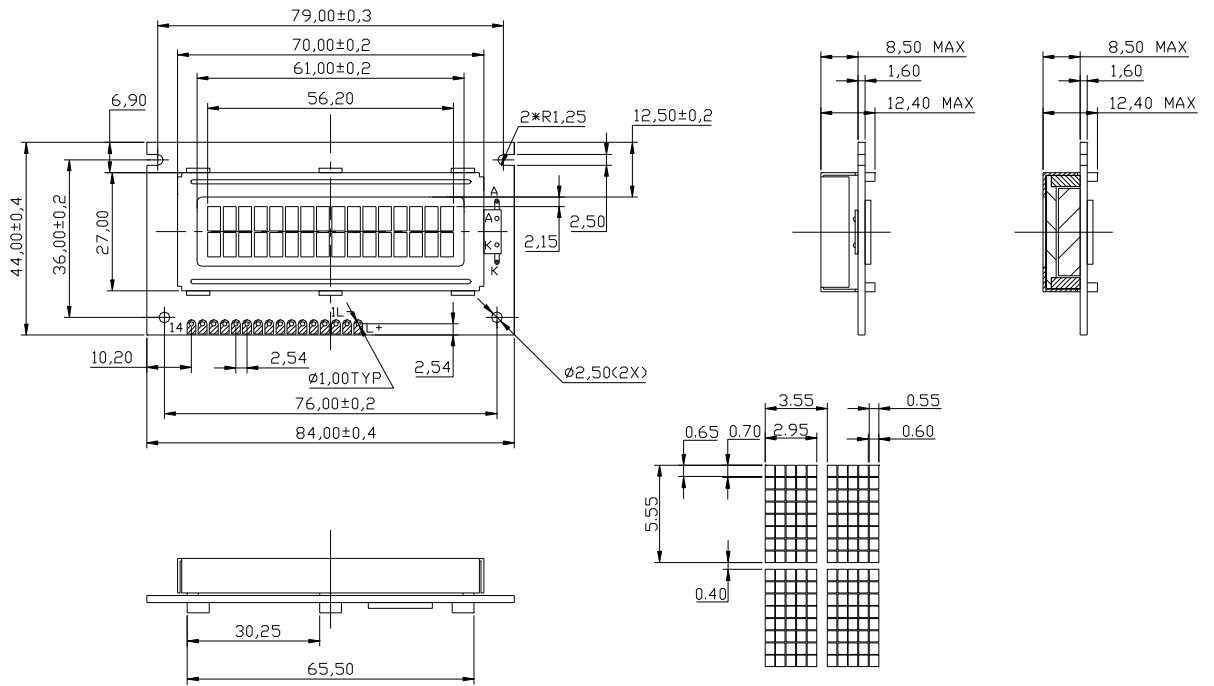
Figure 2.0 External Dimensions For DEM 16217 FGH-LR
