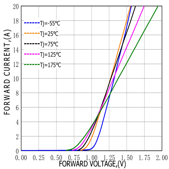
FIG.1-FORWARD CHARACTERISTICS
