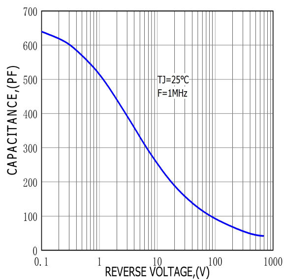
FIG.4-CAPACITANCE VS REVERSE VOLTAGE
