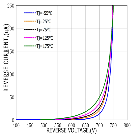
FIG.2-REVERSE CHARACTERISTICS
