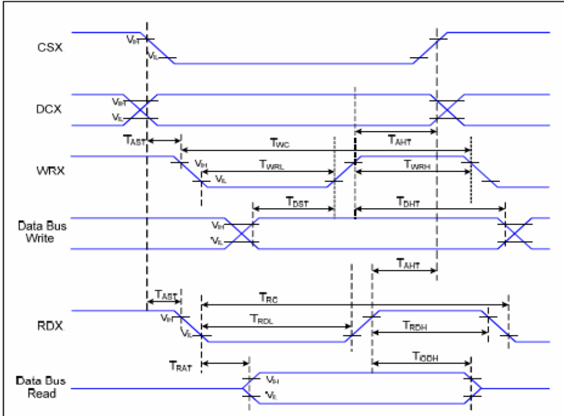
Figure 1 Parallel interface 8080-series Timing Characteristics
