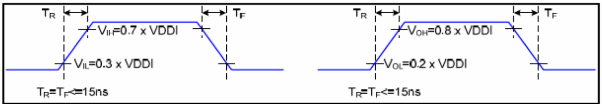
Figure 2 Rising and Falling Timing for I/O Signal
