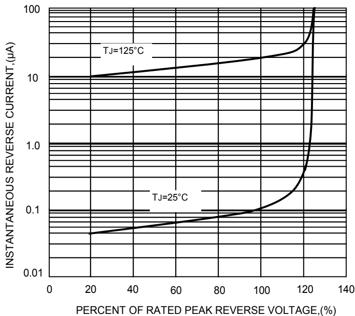
FIG.5-TYPICAL REVERSE CHARACTERISTICS
