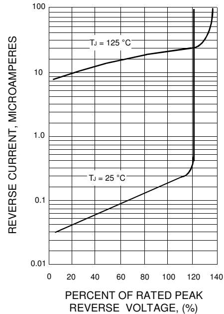
FIG.4 - TYPICAL REVERSE CHARACTERISTICS PER BRIDGE ELEMENT
