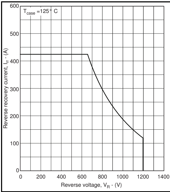
Fig.7 RBSOA
