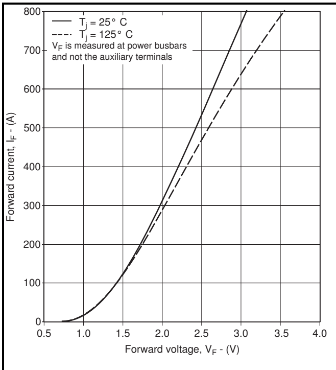
Fig.3 Diode Typical forward characteristics
