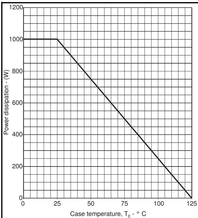
Fig.5 Power dissipation
