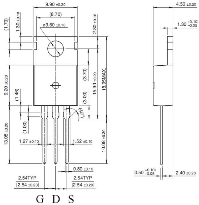
TO-220
