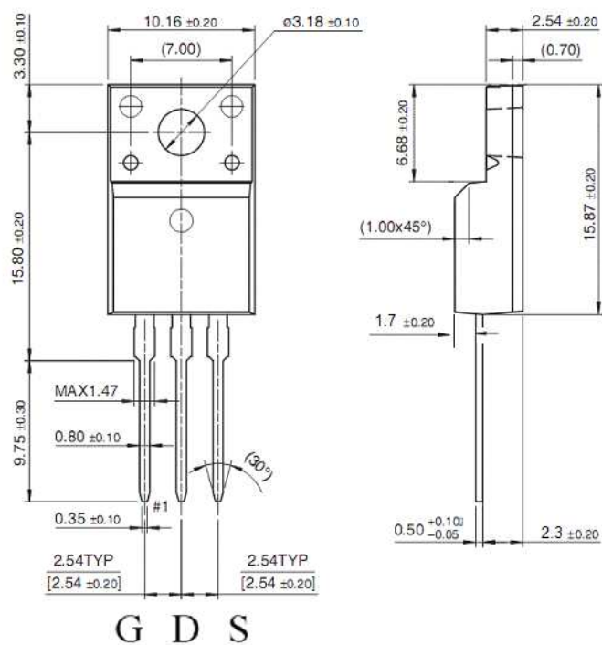
TO-220F
