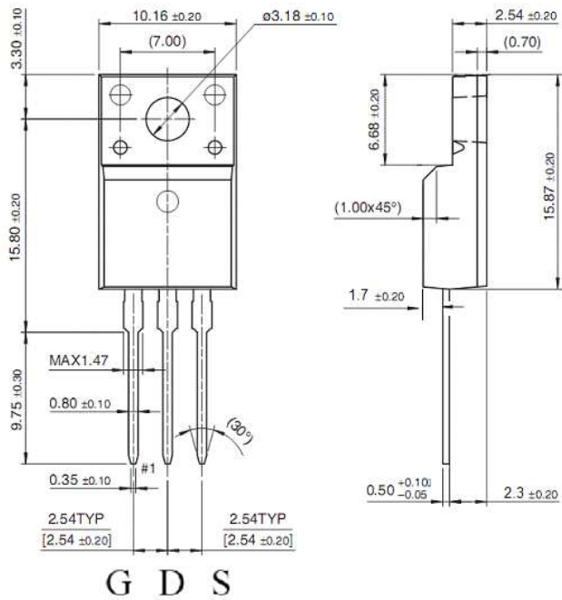
TO-220F
