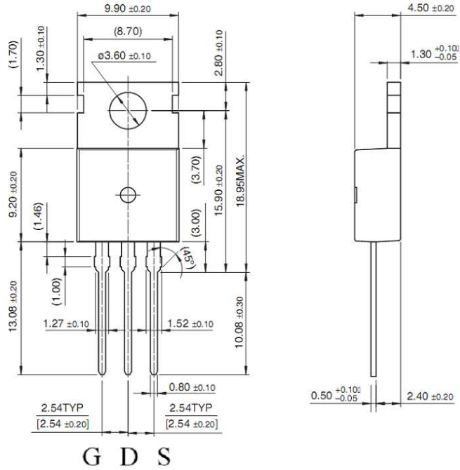
TO-220
