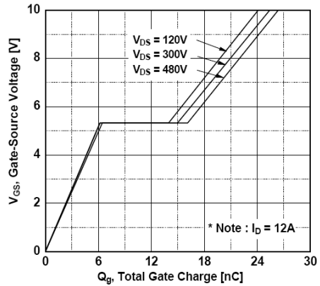
图6. 栅电荷特性曲线 Fig. 6 Gate Charge Characteristics
