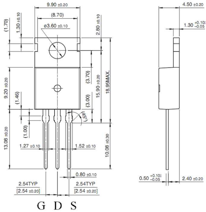
TO-220
