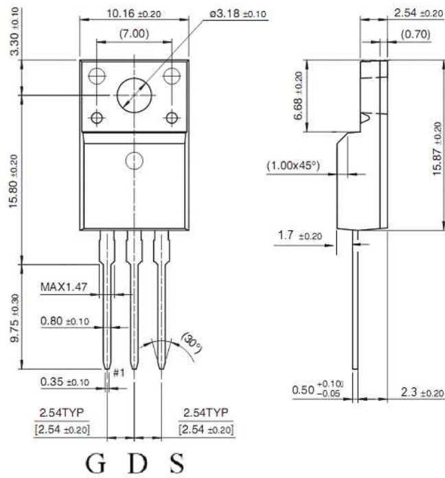
TO-220F
