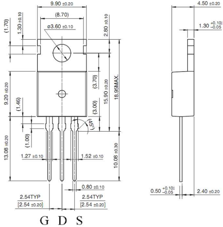
TO-220
