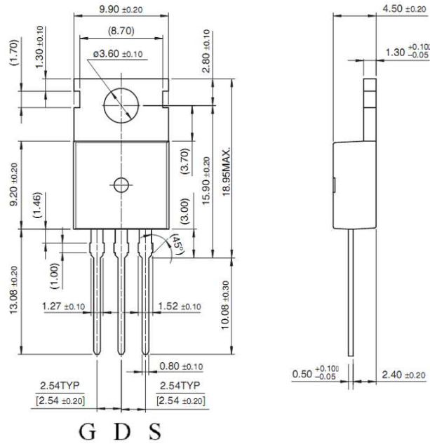
TO-220
