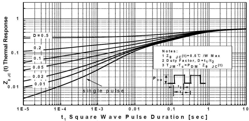
图11. 瞬态热响应曲线(TO-247) Fig. 11 Transient Thermal Response Curve (TO-247)
