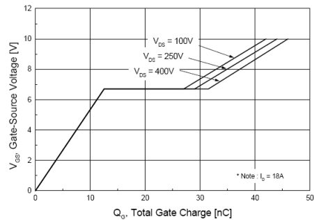
图6. 栅电荷特性曲线 Fig. 6 Gate Charge Characteristics
