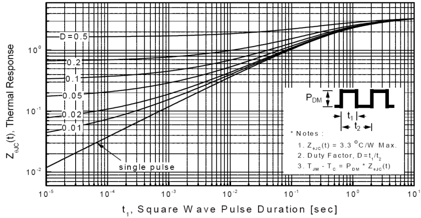
图9. 瞬态热响应曲线(TO-220F) Fig. 9 Transient Thermal Response Curve (TO-220F)
