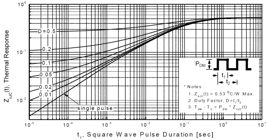
图10. 瞬态热响应曲线(TO-3PN) Fig. 10 Transient Thermal Response Curve (TO-3PN)
