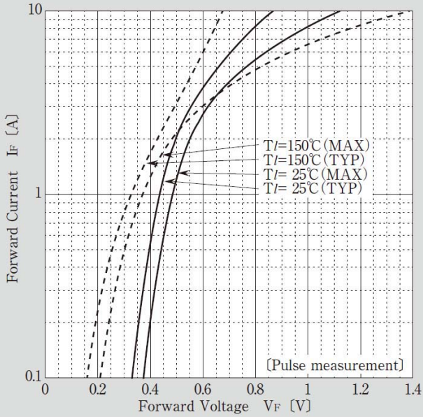
Forward Voltage
